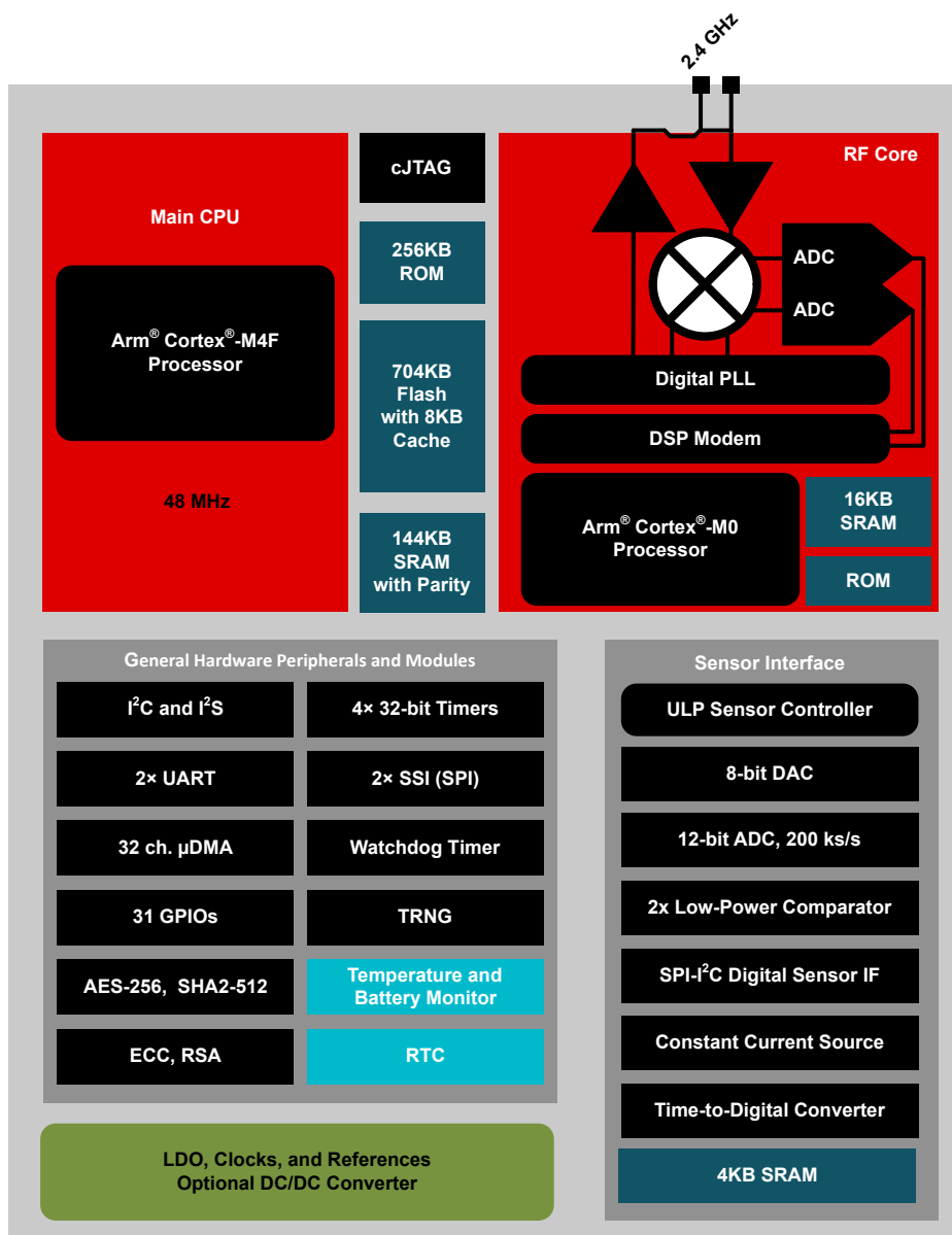
Figure 3-1. CC2652R7 Block Diagram
