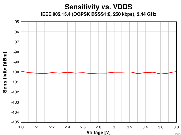
Figure 7-16. Sensitivity vs. Supply Voltage (VDDS) (250 kbps, 2.44 GHz)
