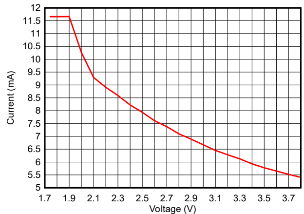
Figure 7-9. RX Current vs Supply Voltage (VDDSD) (BLE 1Mbps, 2.44GHz)
