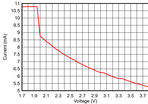
Figure 7-6. Active Mode (MCU) Current vs Supply Voltage (VDDSD) (Running CoreMark)
