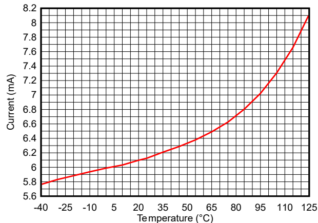
Figure 7-8. RX Current vs Temperature (BLE 1Mbps, 2.44GHz), VDDSD = 3.3V
