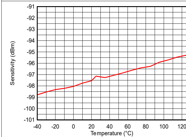
Figure 7-16. Sensitivity vs Temperature (LE 1M PHY, 2.44GHz)
