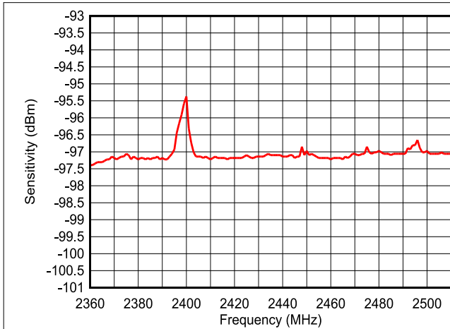
Figure 7-14. Sensitivity vs Frequency (LE 1M PHY)
