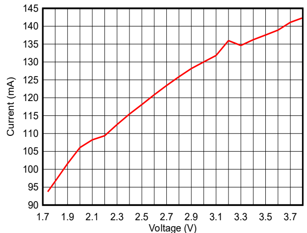
Figure 7-13. TX Current vs Supply Voltage (VDDS) (LE 1M PHY, 2.44GHz, +20dBm)
