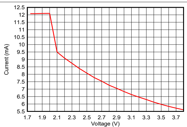
Figure 7-9. RX Current vs Supply Voltage (VDD5) (LE 1M PHY, 2.44GHz)
