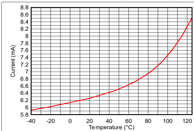
Figure 7-8. RX Current vs Temperature (LE 1M PHY, 2.44GHz), VDD5 = 3.3V
