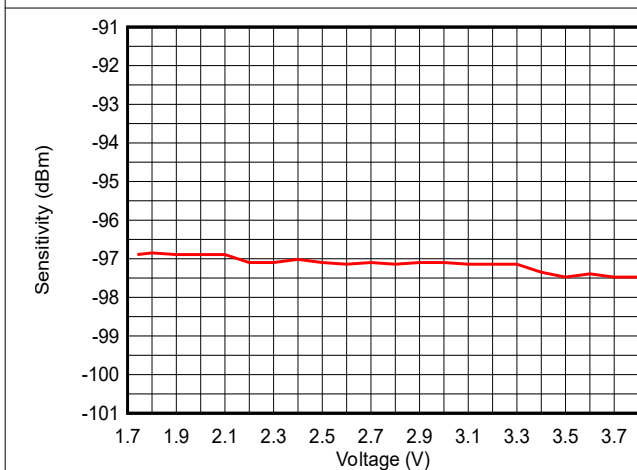
Figure 7-18. Sensitivity vs Supply Voltage (VDDDS) (LE 1M PHY, 2.44GHz)
