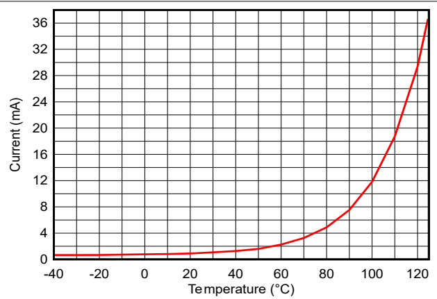
Figure 7-7. Standby Mode (MCU) Current vs Temperature (SRAM and partial register retention, RTC enabled), VDD5 = 3.3V
