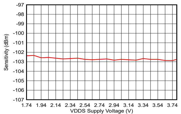
Figure 7-19. Sensitivity vs VDDDS (IEEE 802.15.4 PHY)
