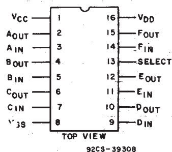
TERMINAL ASSIGNMENT
