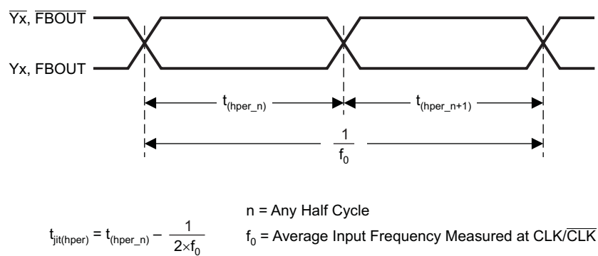
Figure 8. Half-Period Jitter
