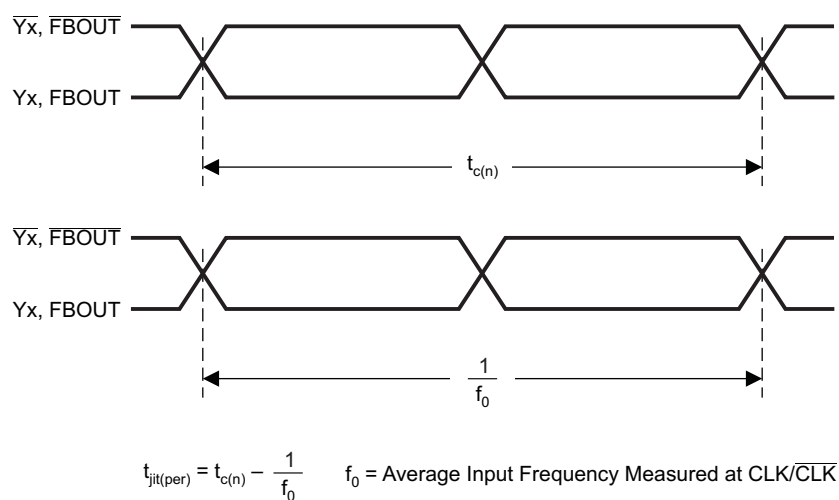
Figure 7. Period Jitter
