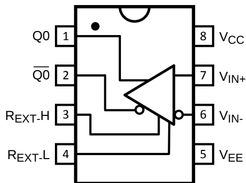
Figure 2. 8-Pin SOIC See Package Number D
