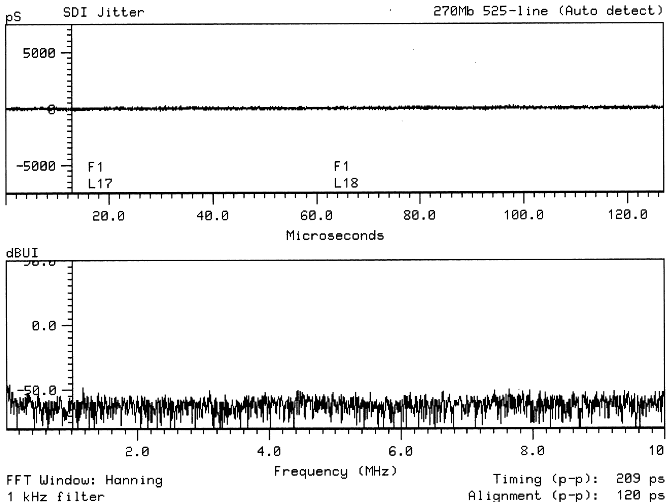
Figure 12. Jitter Plots
