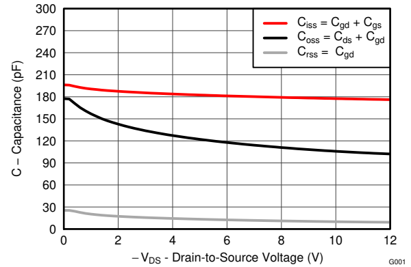
Figure 5-5. Capacitance
