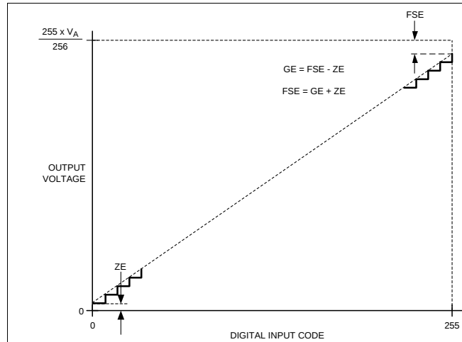
Figure 2. I/O Transfer Characteristic
