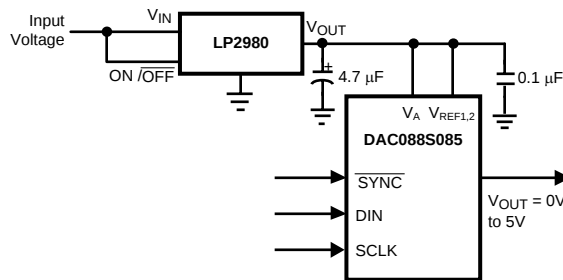
Figure 46. Using the LP2980 Regulator
