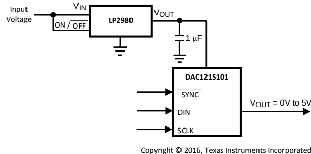
Figure 42. Using the LP2980-N Regulator
