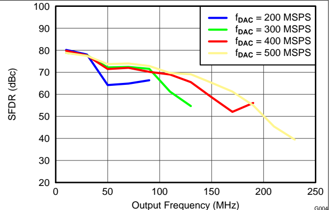
Figure 10. SFDR vs Output Frequency Over f_{DAC}
