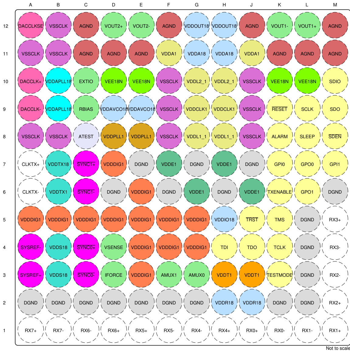
Figure 5-1. DAC38RF83, DAC38RF85 AAV Package 144-Pin (FCBGA) 144-Pin FCBGA Top View
