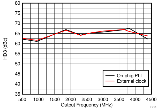
D014 DAC38RF83/93/85
