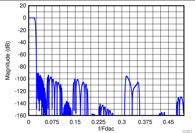
Figure 41. Composite Magnitude Response for 24x Interpolation
