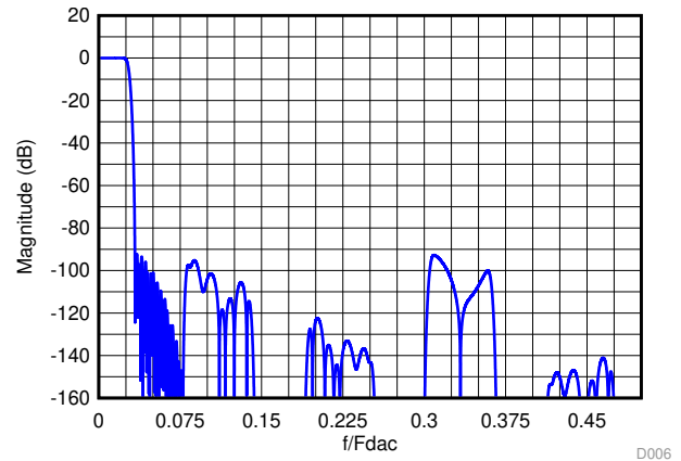
Figure 39. Composite Magnitude Response for 18x Interpolation
