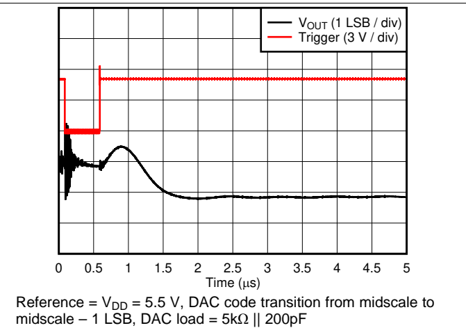
Figure 37. Glitch Impulse, Falling Edge, 1-LSB Step
