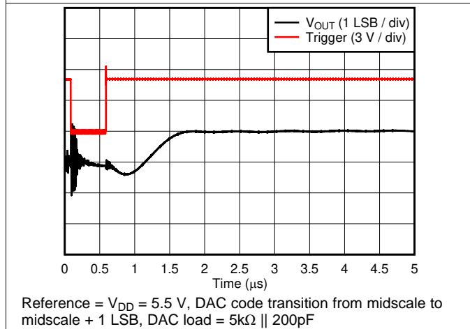
Figure 36. Glitch Impulse, Rising Edge, 1-LSB Step
