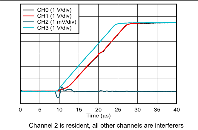
Figure 5-25. Voltage Output Channel-to-Channel Crosstalk
