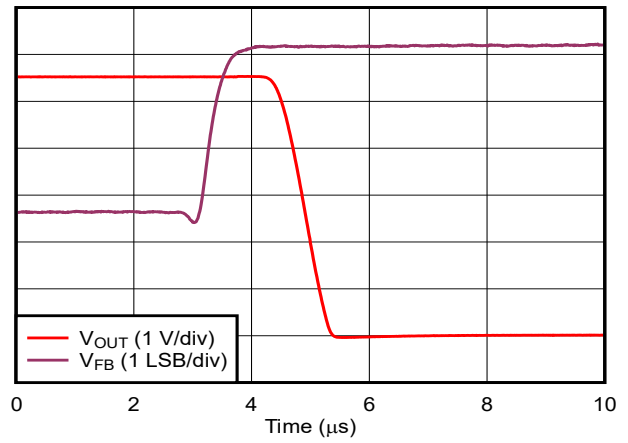
Figure 5-60. Comparator Response Time: High-to-Low Transition
