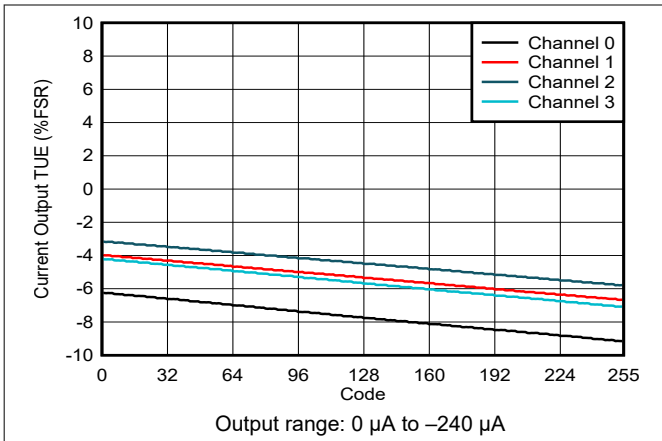
Figure 5-43. Current Output TUE vs Digital Input Code
