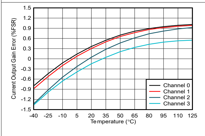
Figure 5-47. Current Output Gain Error vs Temperature
