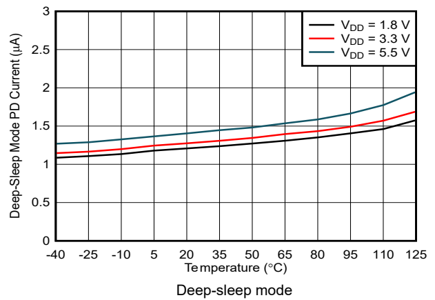
Figure 5-65. Power-Down Current vs Temperature
