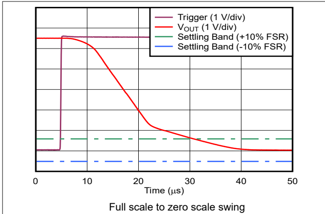
Figure 5-22. Voltage Output Setting Time: Falling Edge
