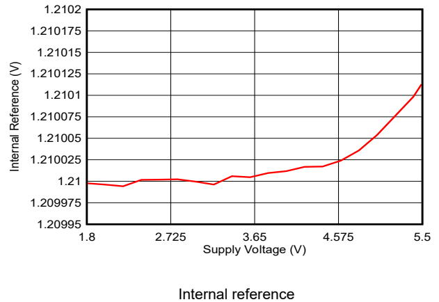
Figure 5-63. Internal Reference vs Supply Voltage
