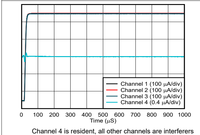
Figure 5-53. Current Output Channel-to-Channel Crosstalk
