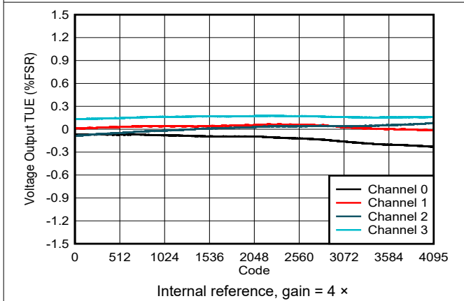
Figure 5-12. Voltage Output TUE vs Digital Input Code
