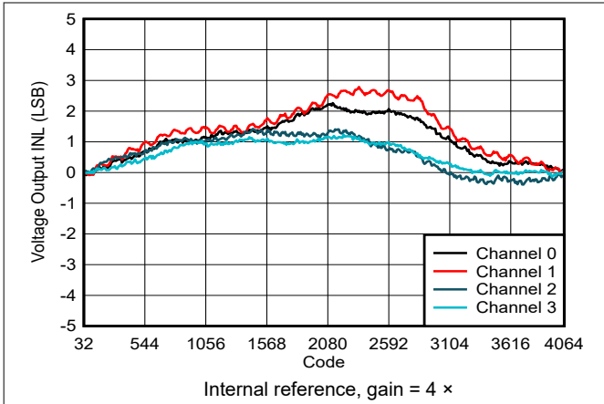
Figure 5-4. Voltage Output INL vs Digital Input Code
