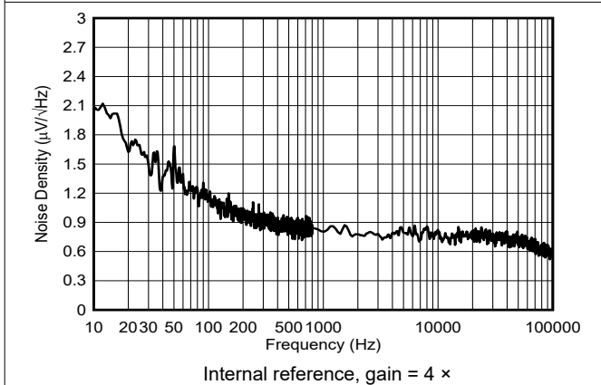
Figure 5-26. Voltage Output Noise Density
