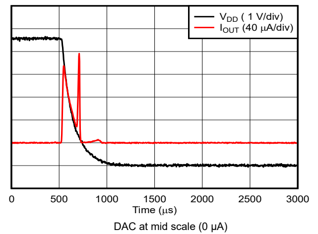
Figure 5-52. Current Output Power-Off Glitch
