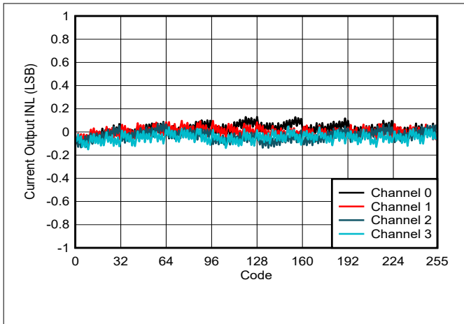
Figure 5-31. Current Output INL vs Digital Input Code
