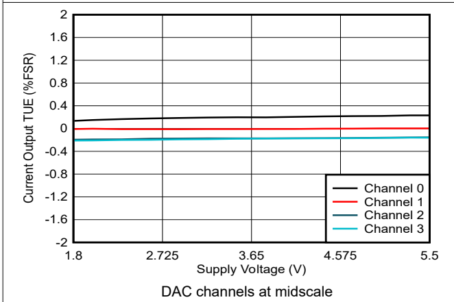
Figure 5-45. Current Output TUE vs Supply Voltage
