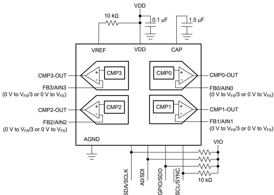
Figure 6-3. Comparator Interface
