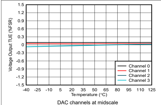
Figure 5-14. Voltage Output TUE vs Temperature
