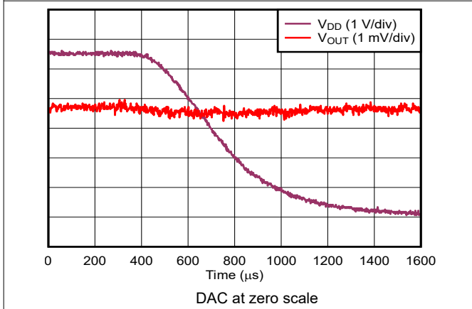
Figure 5-24. Voltage Output Power-Off Glitch
