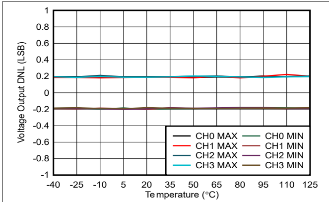
Figure 5-10. Voltage Output DNL vs Temperature
