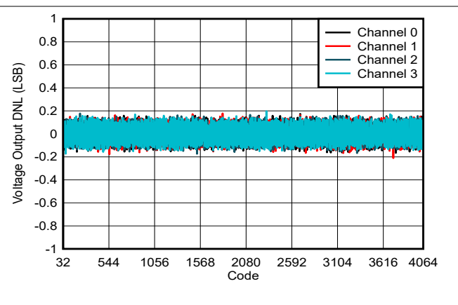
Figure 5-9. Voltage Output DNL vs Digital Input Code
