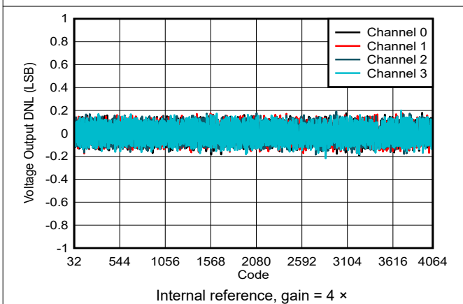
Figure 5-8. Voltage Output DNL vs Digital Input Code
