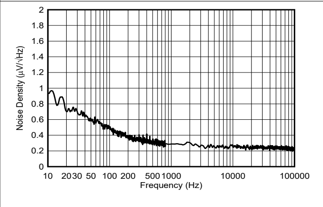
Figure 5-27. Voltage Output Noise Density
