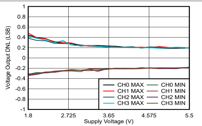
Figure 5-11. Voltage Output DNL vs Supply Voltage
