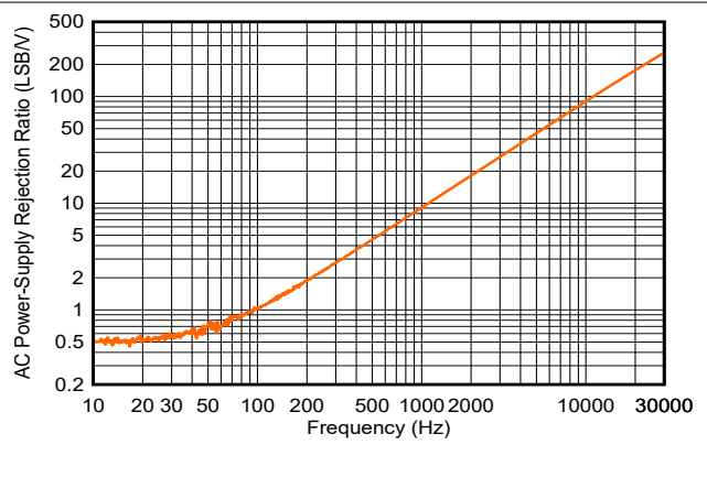
Figure 5-54. Current Output AC PSRR vs Frequency
