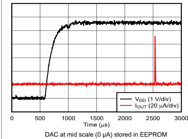
Figure 5-51. Current Output Power-On Glitch
