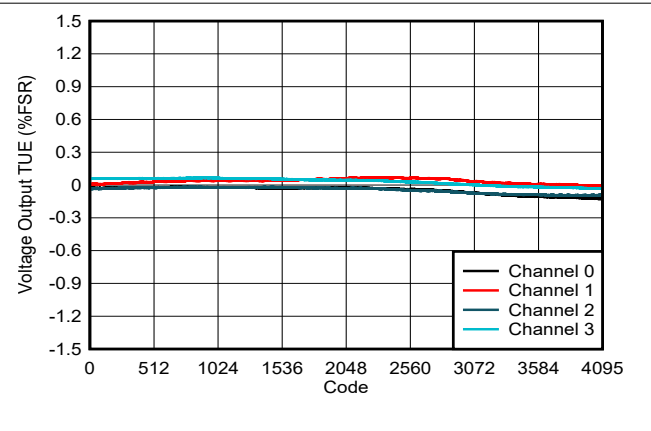
Figure 5-13. Voltage Output TUE vs Digital Input Code
