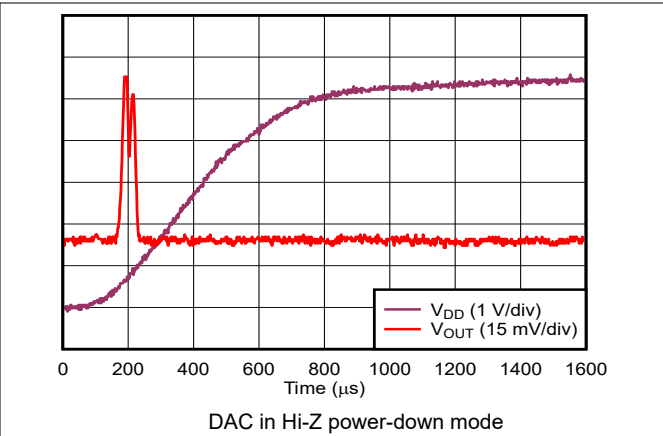
Figure 5-23. Voltage Output Power-On Glitch
