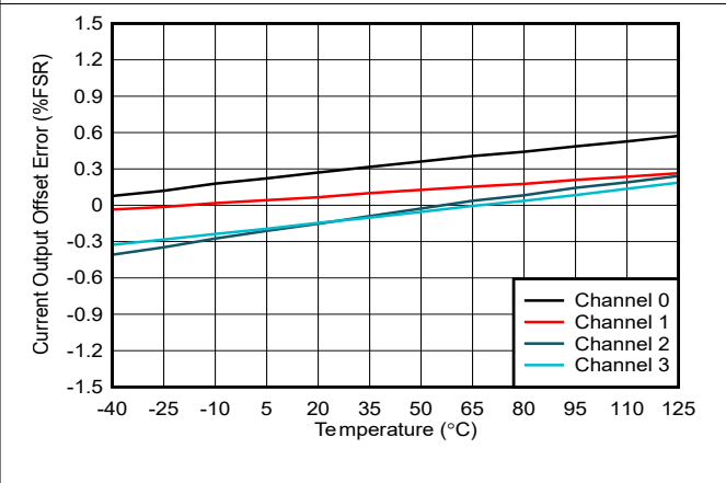
Figure 5-46. Current Output Offset Error vs Temperature
