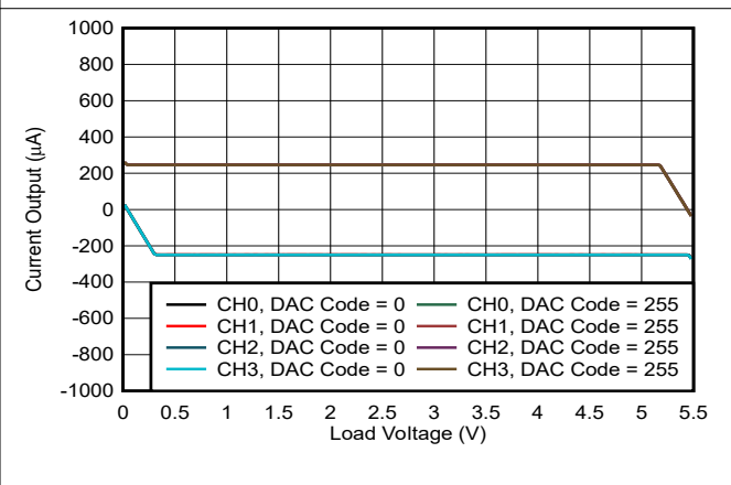
Figure 5-48. Current Output vs Load Voltage
