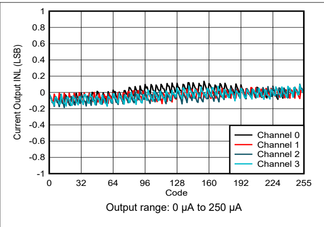
Figure 5-32. Current Output INL vs Digital Input Code
