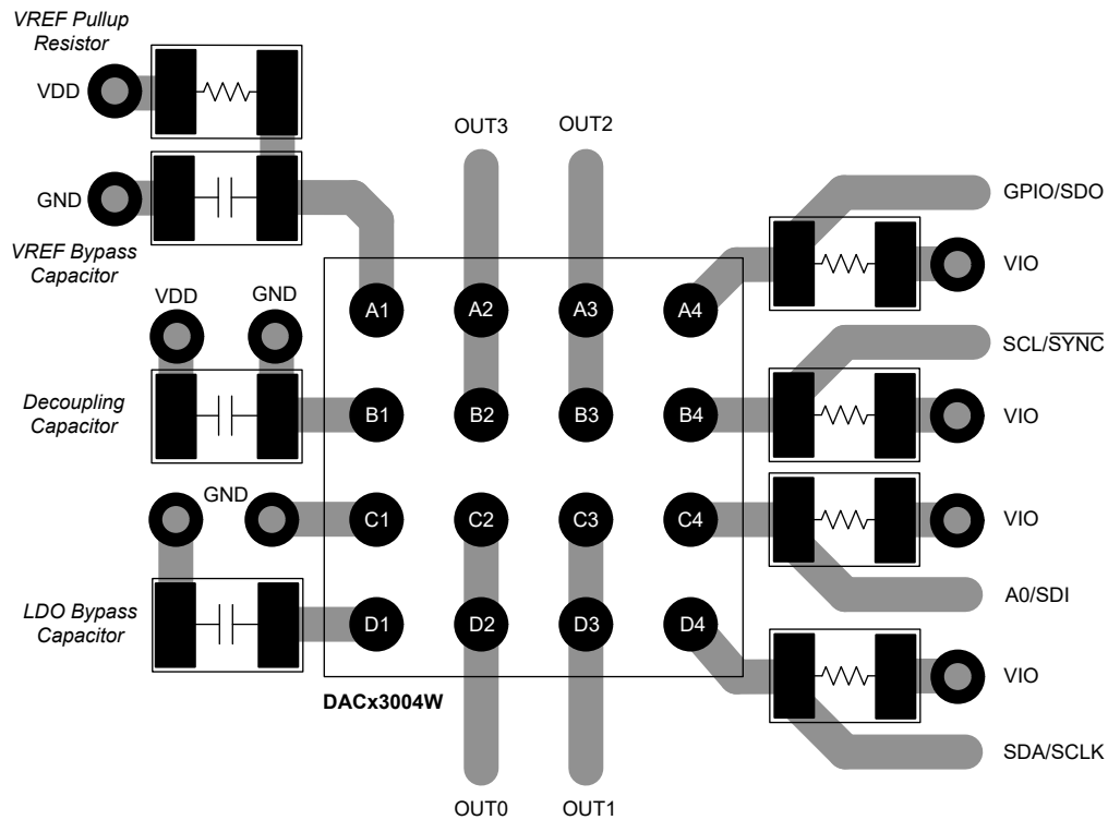
Figure 7-3. Layout Example
