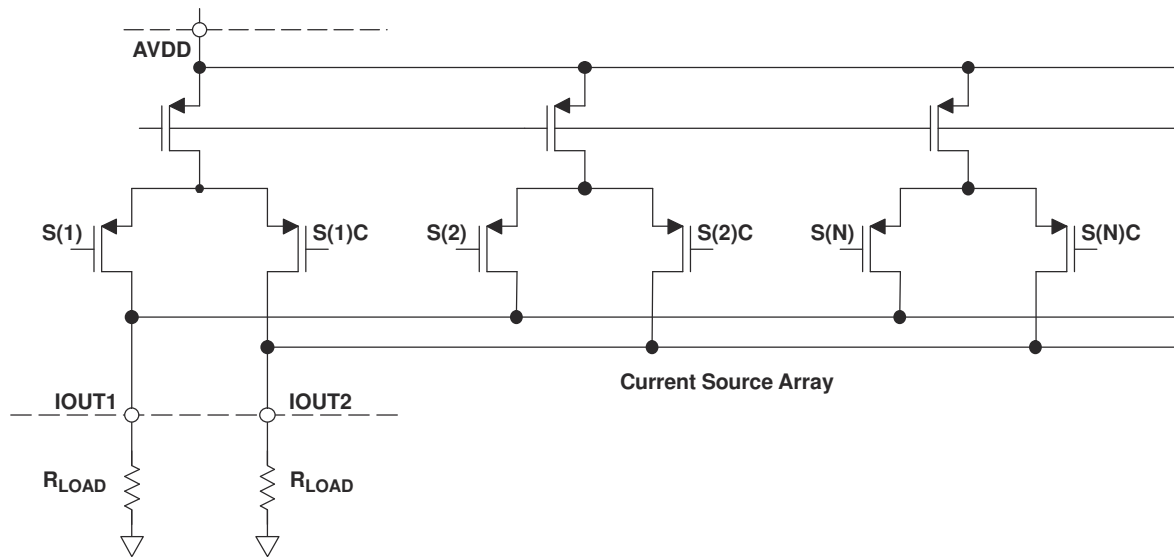
Figure 8-1. Analog Outputs
