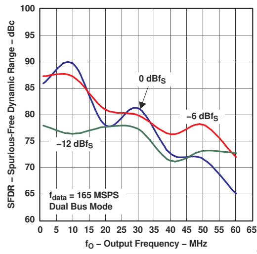
Figure 6-6. Spurious-Free Dynamic Range vs Output Frequency
