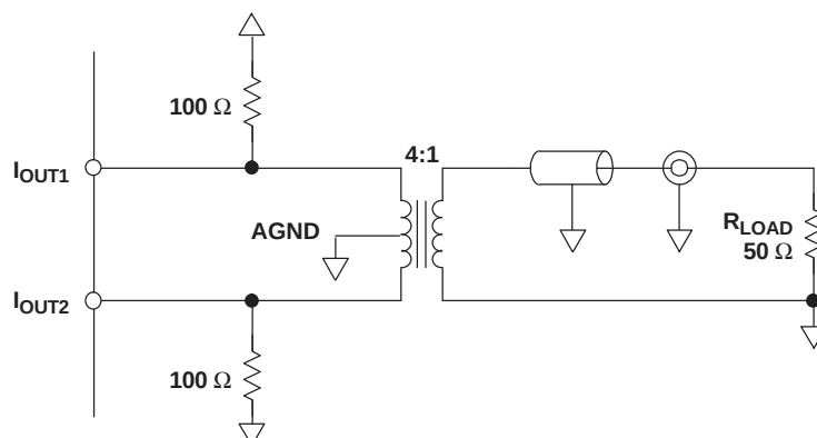
Figure 24. Driving a Doubly-Terminated 50-Ω Cable Using a 4:1 Impedance Ratio Transformer
