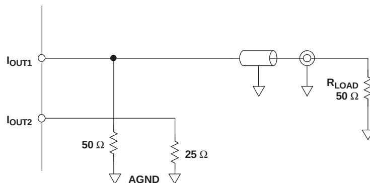
Figure 25. Driving a Doubly-Terminated 50-Ω Cable Using a Single-Ended Output
