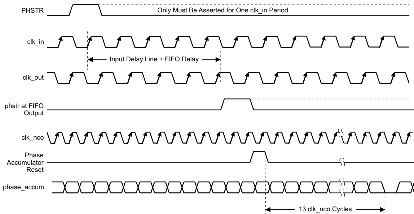
Figure 55. NCO Phase Accumulator Reset Synchronization Timing
