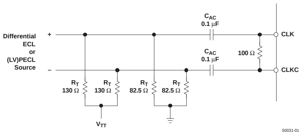
Figure 67. Driving the DAC5687 With Differential ECL/PECL Clock Source
