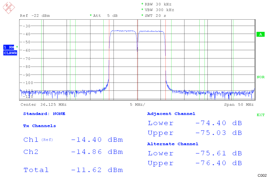
Figure 80. Two QAM256 Carriers With at 36-MHz IF
