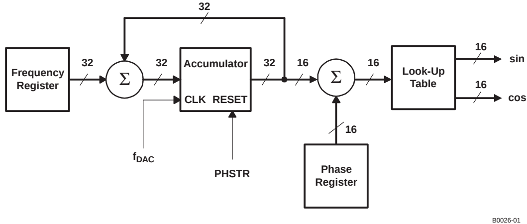
Figure 40. Block Diagram of the NCO
