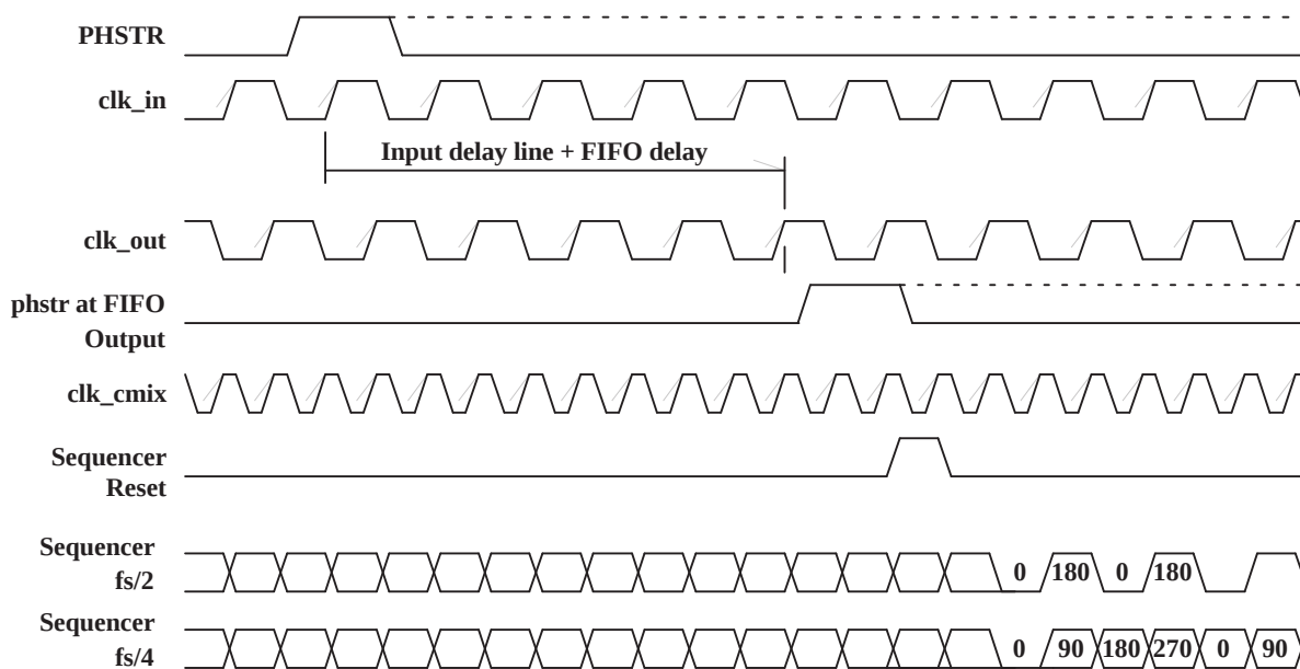
Figure 55. CMIX Reset Synchronization Timing
