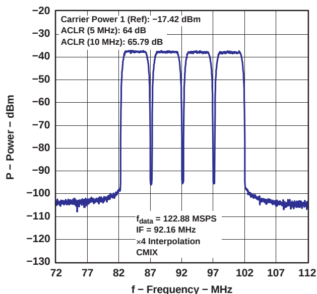
Figure 23. WCDMA TM1 : Four Carrier, PLL On, DVDD = 1.8 V
