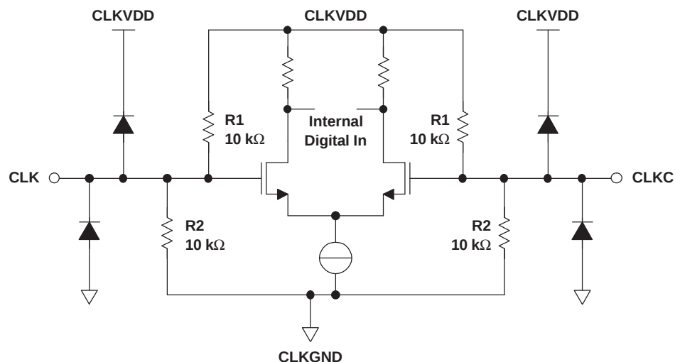
Figure 62. Clock Input Equivalent Circuit
