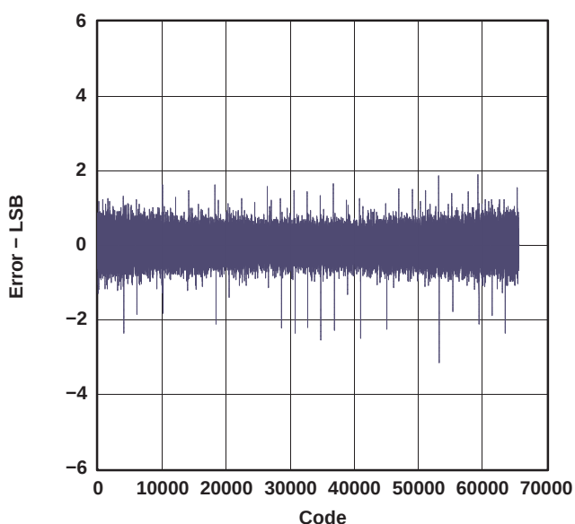
Figure 3. Differential Nonlinearity
