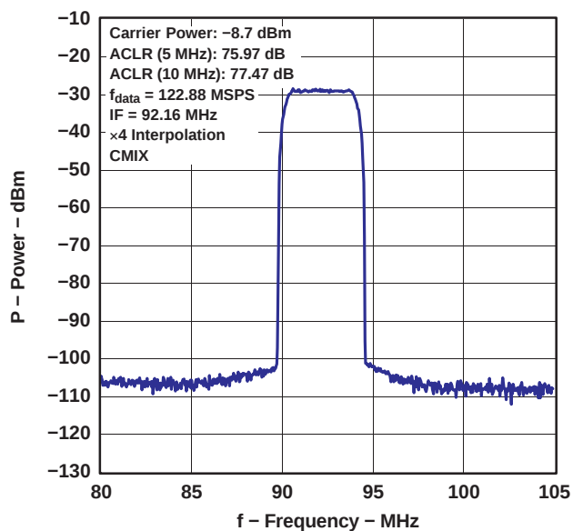
Figure 16. WCDMA TM1 : Single Carrier, PLL Off, DVDD = 1.8 V
