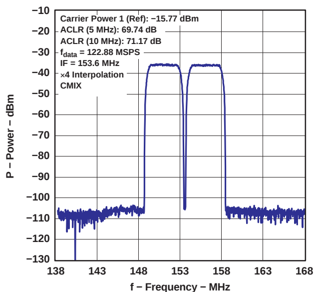
Figure 25. WCDMA TM1 : Two Carrier, PLL Off, DVDD = 2.1 V
