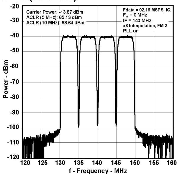
Figure 18. WCDMA TM1: Four Carriers, PLL On
