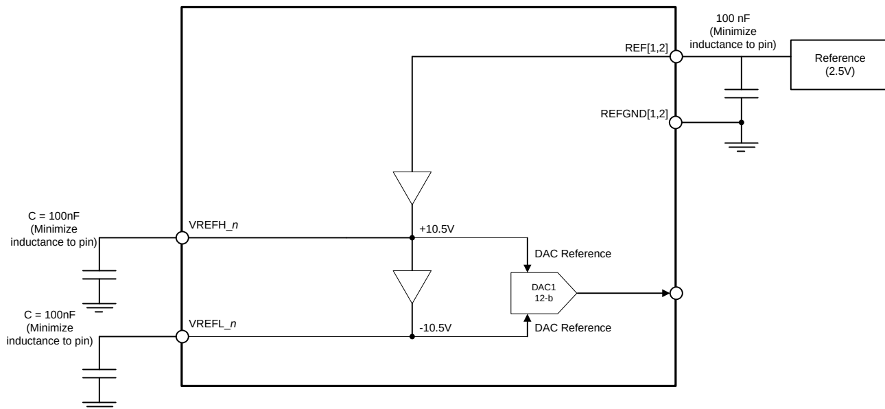
Figure 34. Reference Operation
