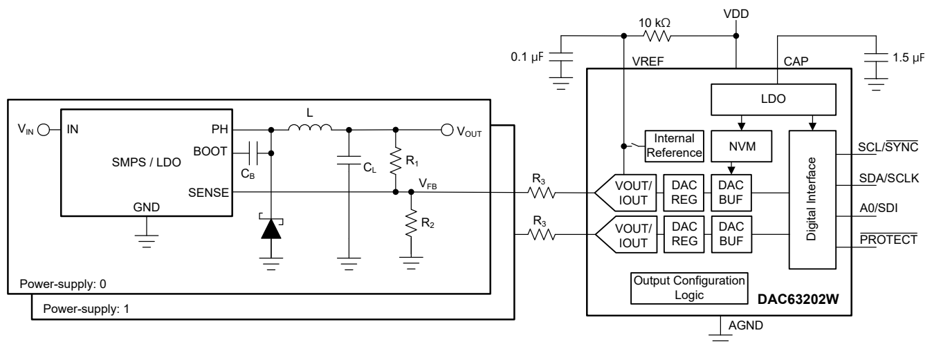
Figure 7-1. Voltage Margining and Scaling
