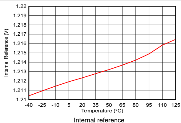
Figure 5-52. Internal Reference vs Temperature
