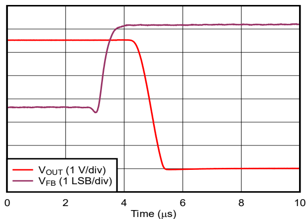
Figure 5-50. Comparator Response Time: High-to-Low Transition
