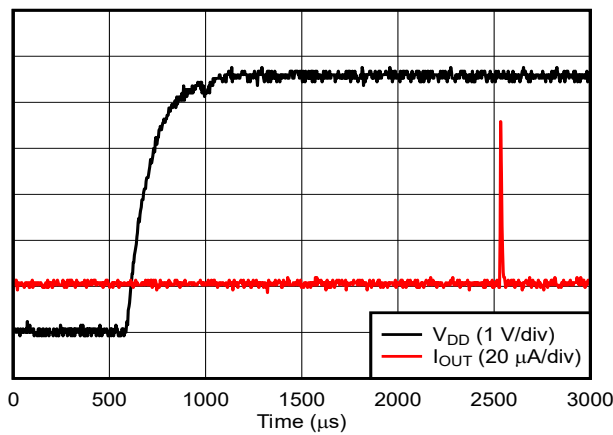
Figure 5-42. Current Output Setting Time, Rising Edge
