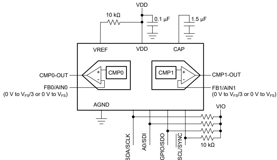
Figure 6-3. Comparator Interface
