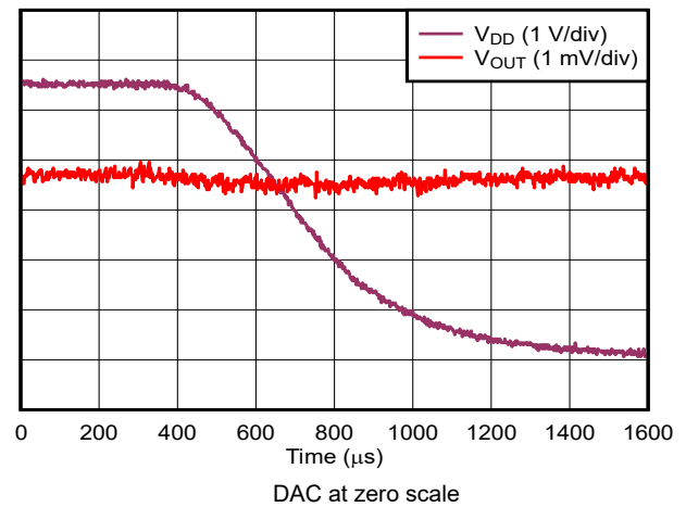
Figure 5-25. Voltage Output Power-Off Glitch
