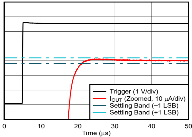
Figure 5-42. Current Output Setting Time, Rising Edge
