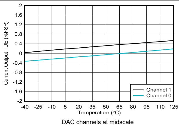
Figure 5-37. Current Output TUE vs Temperature
