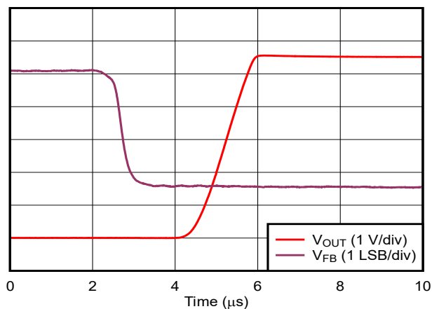
Figure 5-49. Comparator Response Time: Low-to-High Transition
