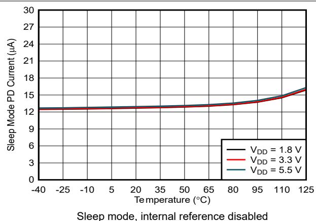
Figure 5-54. Power-Down Current vs Temperature
