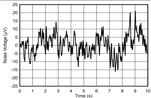
Figure 5-29. Voltage Output Flicker Noise
