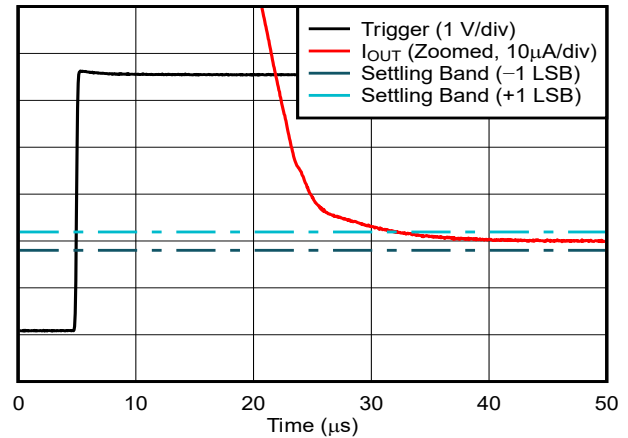
Figure 5-43. Current Output Setting Time, Falling Edge
