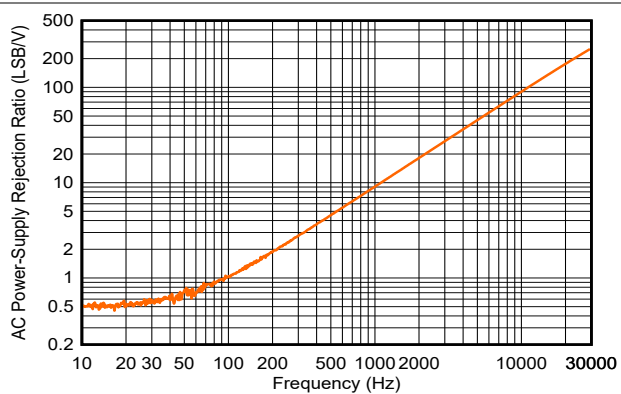
Figure 5-48. Current Output AC PSRR vs Frequency
