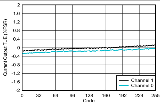
Figure 5-36. Current Output TUE vs Digital Input Code
