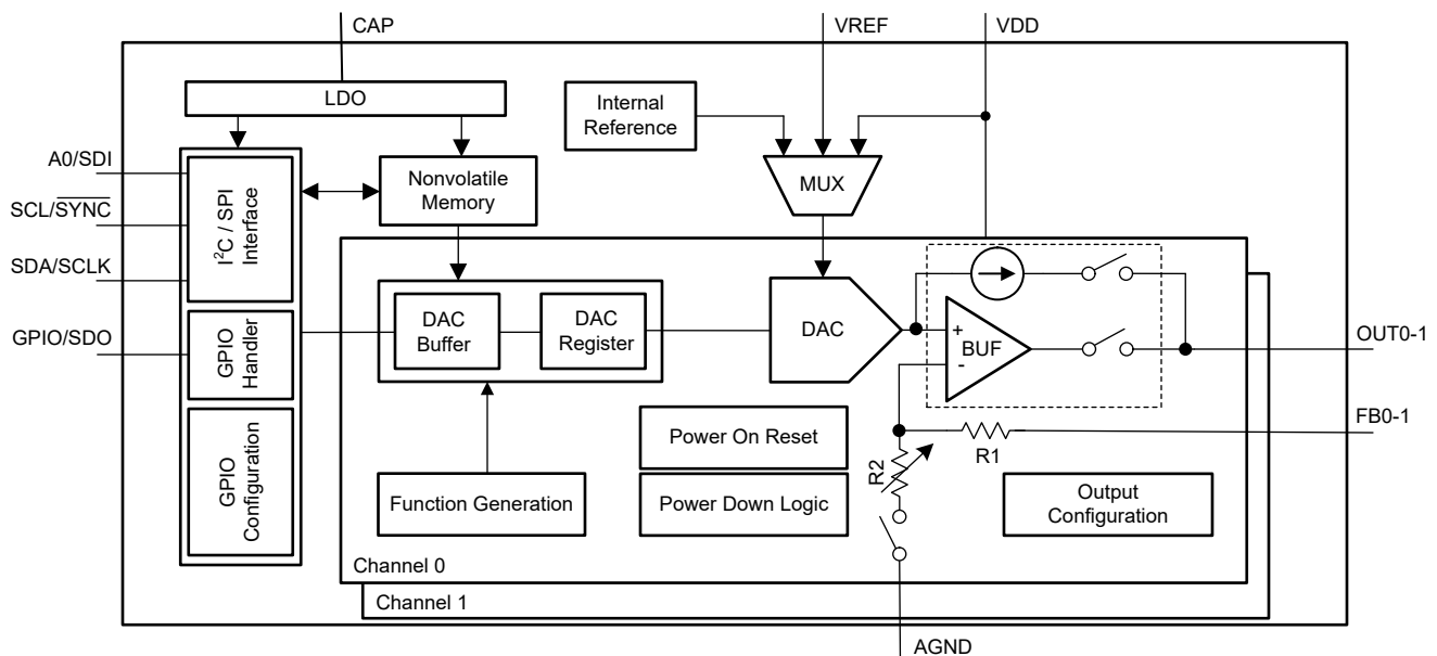
Figure 6-1. Functional Block Diagram
