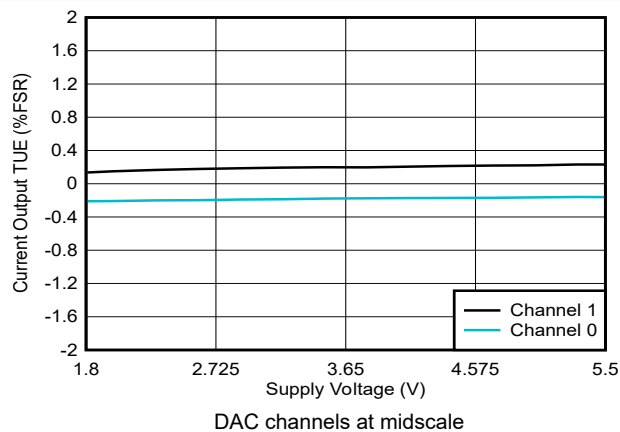
Figure 5-38. Current Output TUE vs Supply Voltage
