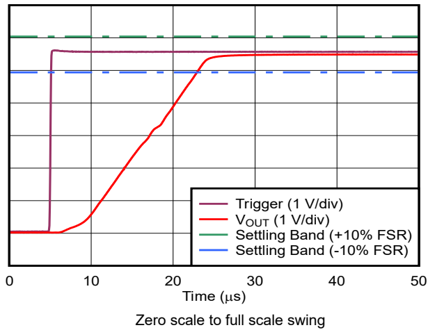
Figure 5-22. Voltage Output Setting Time - Rising Edge
