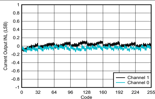
Figure 5-30. Current Output INL vs Digital Input Code
