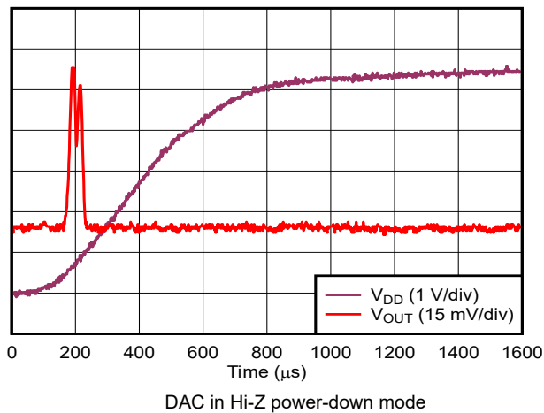
Figure 5-24. Voltage Output Power-On Glitch
