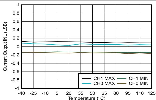
Figure 5-31. Current Output INL vs Temperature
