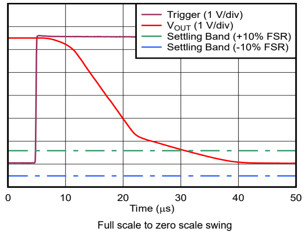
Figure 5-23. Voltage Output Setting Time - Falling Edge
