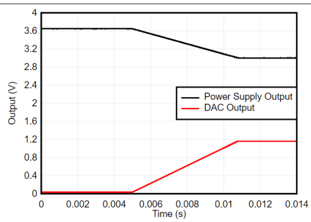
Figure 7-3. Power-Supply Margin Low
