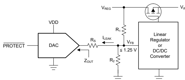
Figure 6-9. High-Impedance (Hi-Z) Output and PROTECT Input
