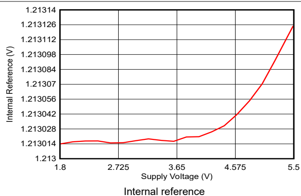
Figure 5-53. Internal Reference vs Supply Voltage
