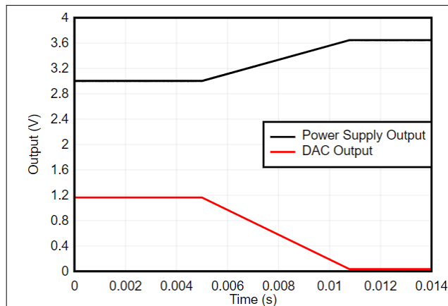
Figure 7-2. Power-Supply Margin High
