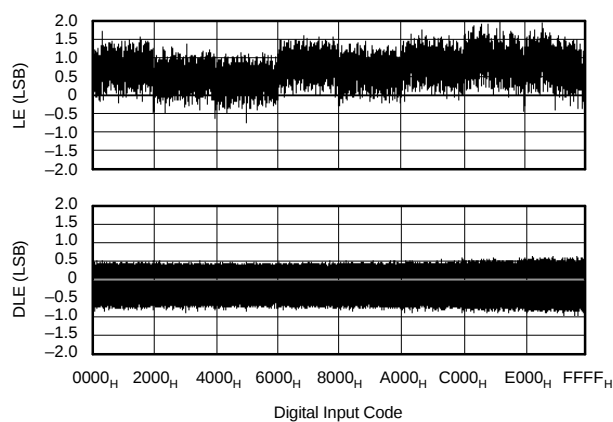
Figure 55. Integral Linearity and Differential Linearity Error Curves for Figure 56
