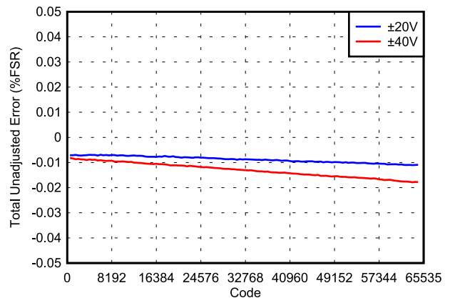
Figure 8-7. TUE vs Digital Input Code (Bipolar Mode)
