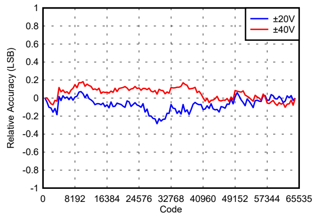
Figure 8-5. Relative Accuracy vs Digital Input Code (Bipolar Mode)
