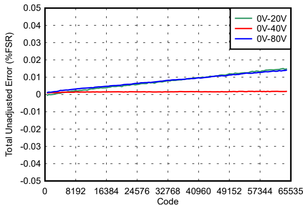
Figure 8-6. TUE vs Digital Input Code (Unipolar Mode)
