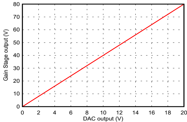
Figure 8-2. Gain Stage Output vs DAC Output (Unipolar Mode)
