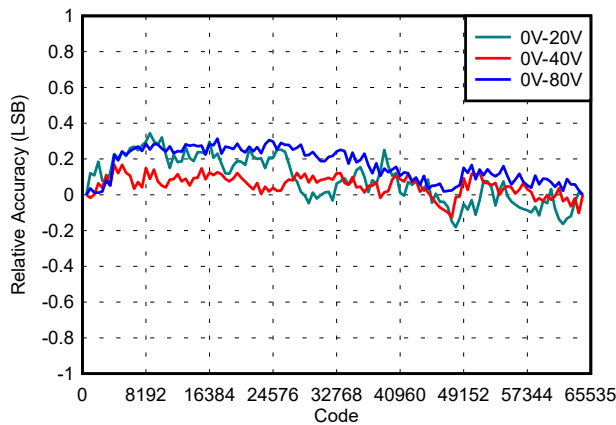
Figure 8-4. Relative Accuracy vs Digital Input Code (Unipolar Mode)
