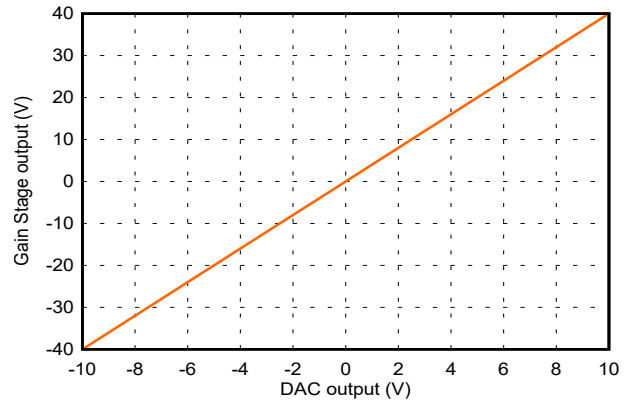
Figure 8-3. Gain Stage Output vs DAC Output (Bipolar Mode)
