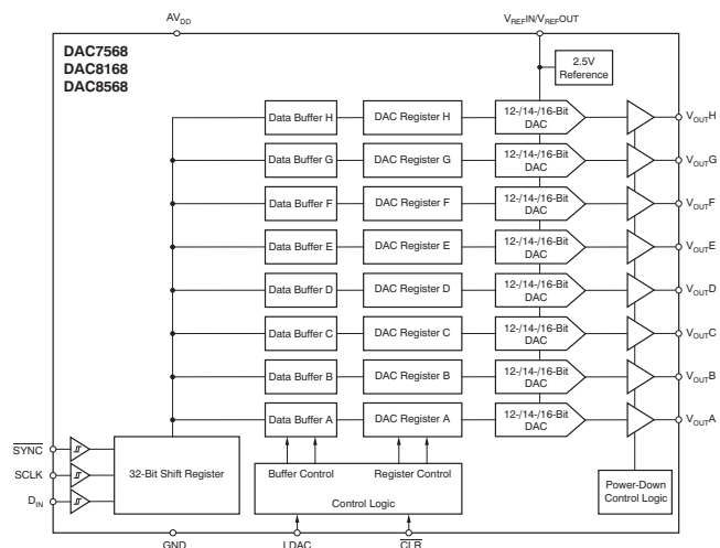
Block Diagram
