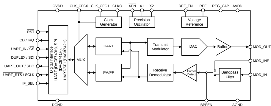
Simplified Schematic
