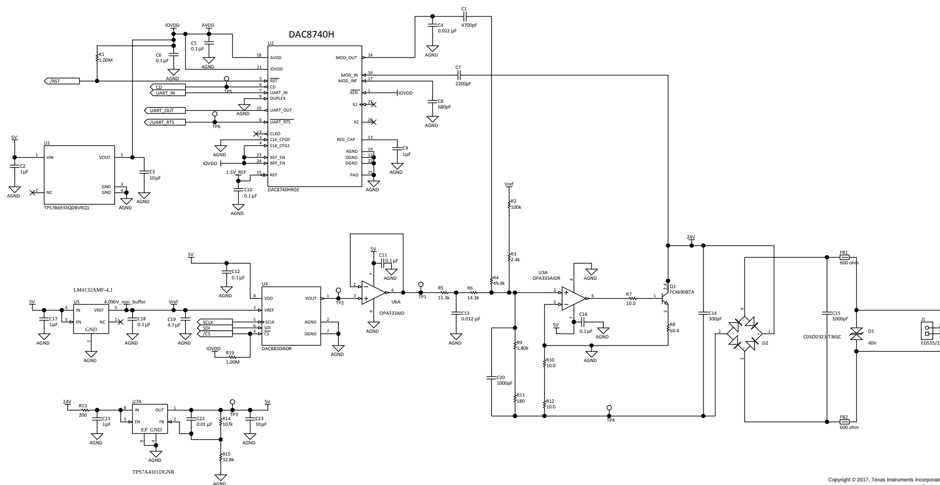
Figure 34. 2-Wire Transmitter with DAC8742H HART Modem Design Schematic
