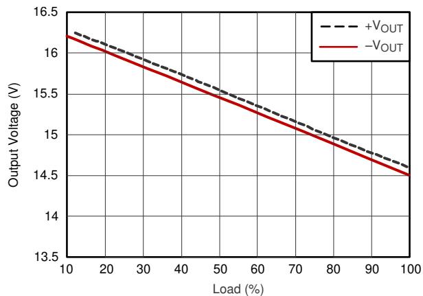
Figure 6-26. Load Regulation
