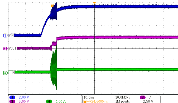
Figure 7-5. DCP010505BP Start-Up at 100% Load
