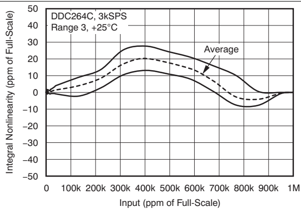
Figure 1. Integral Nonlinearity
