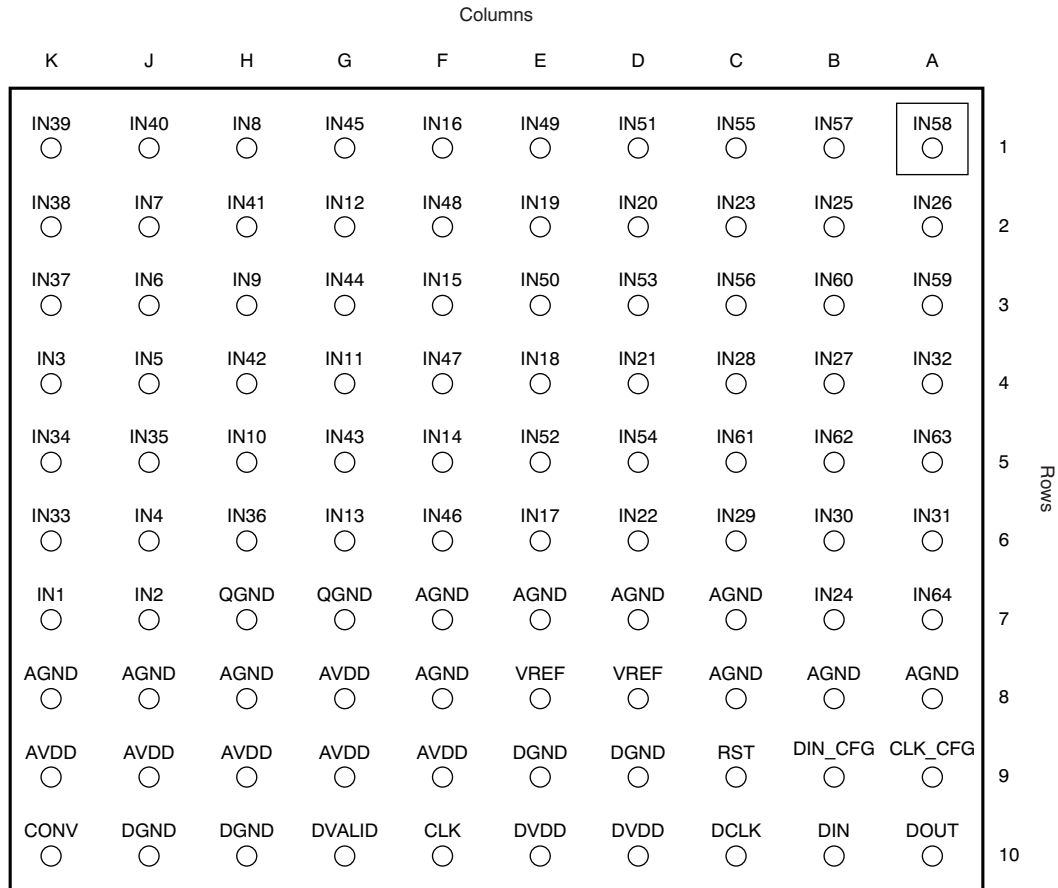
Pin Functions
