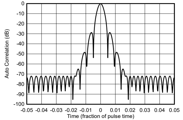
Figure 8-16. Auto-correlation of NLFM Chirp
