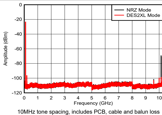
Figure 6-28. Dual Tone, f_{\text{OUT}} = 97\text{MHz} , -12dBFS
