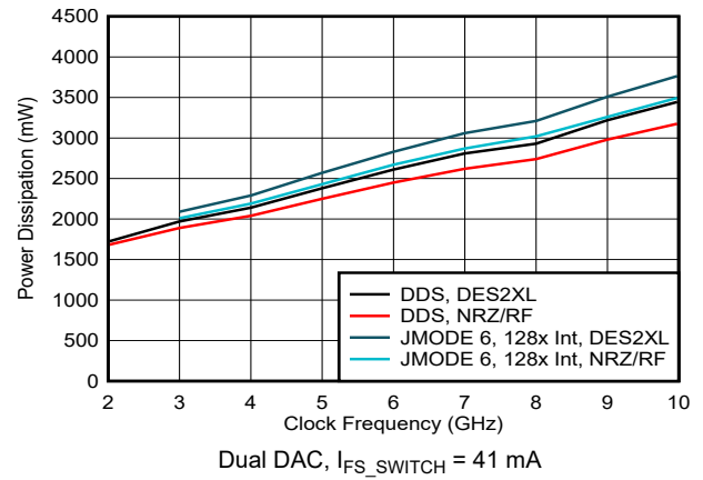
Figure 6-45. Power Dissipation vs Clock Frequency and Digital Mode
