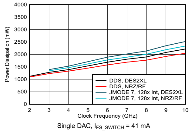
Figure 6-47. Power Dissipation vs Clock Frequency and Digital Mode
