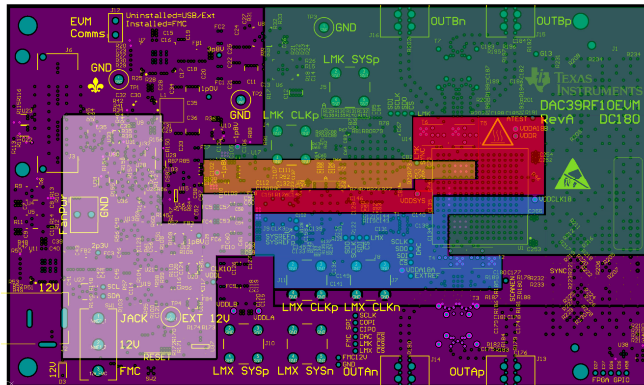
Layer12 / PWR3 DAC VDDA18A = RED DAC VDDA18B = ORANGE DAC VDDB = YELLOW DAC VEEa = GREEN DAC VEEb = BLUE VDDIO = WHITE Figure 8-32. Power Plane Layout for Layer 12
