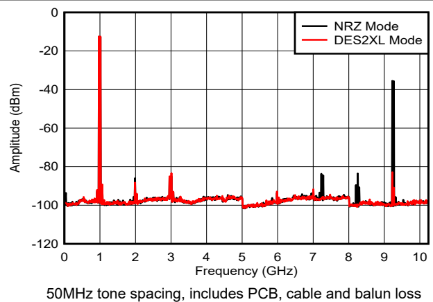
Figure 6-29. Dual Tone, f_{\text{OUT}} = 997\text{MHz} , 0dBFS
