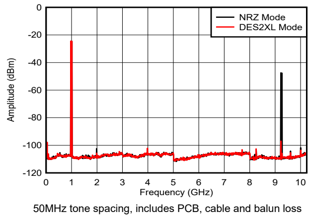
Figure 6-31. Dual Tone, f_{\text{OUT}} = 997\text{MHz} , -12dBFS
