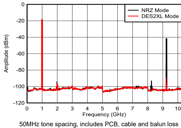
Figure 6-30. Dual Tone, f_{\text{OUT}} = 997\text{MHz} , -6dBFS
