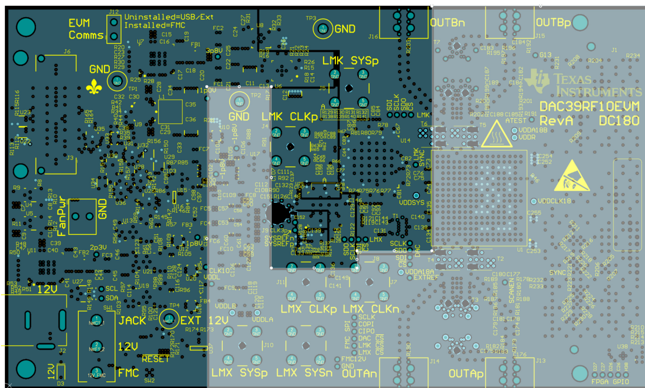
Layer3 / PWR1 DAC DVDD = WHITE Other PWR Planes = AUX Supplies Figure 8-30. Power Plane Layout for Layer 3
