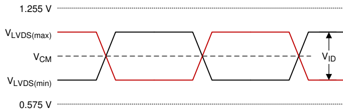
Figure 6-10. SubLVDS Waveform Parameters
