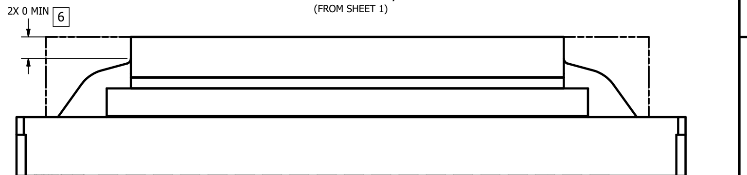
VIEW D ENCAPSULANT MAXIMUM HEIGHT
