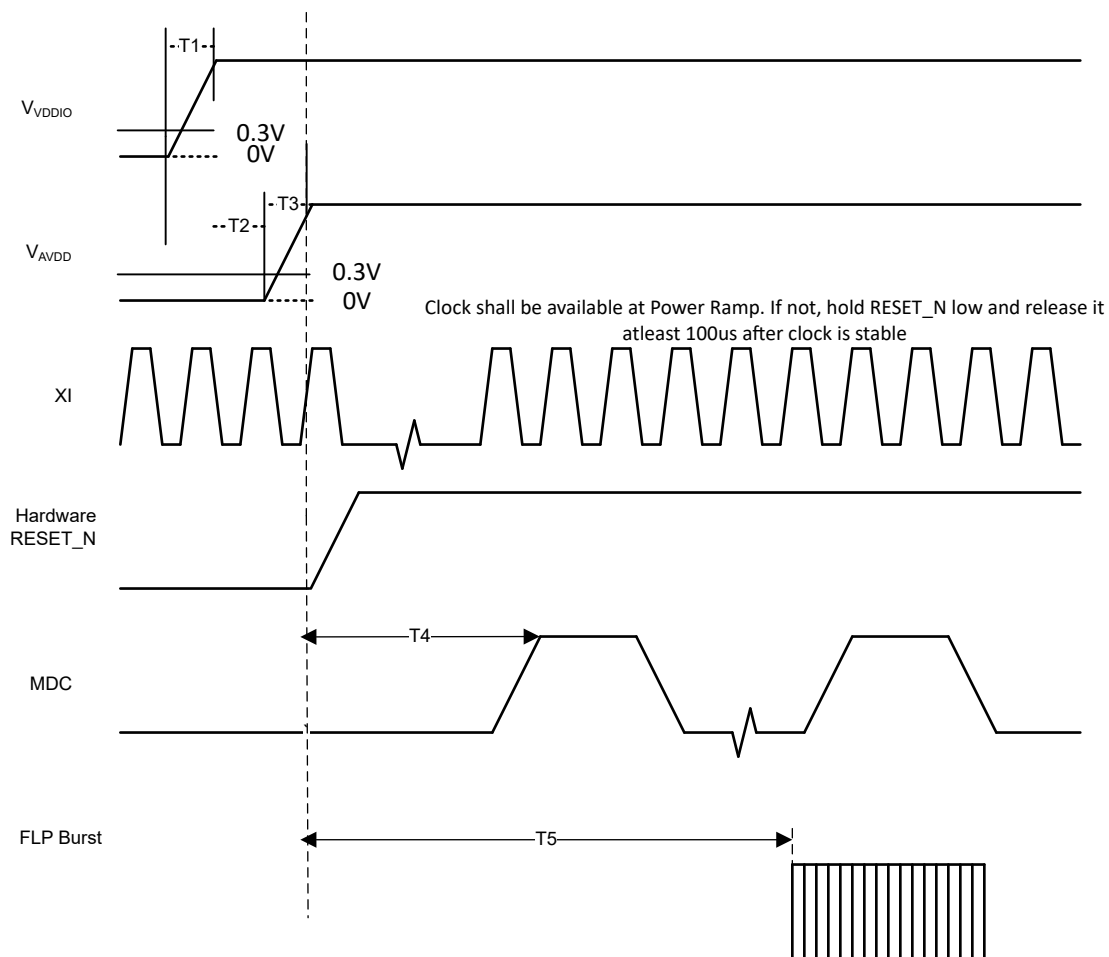
Figure 5-1. Power-Up Timing
