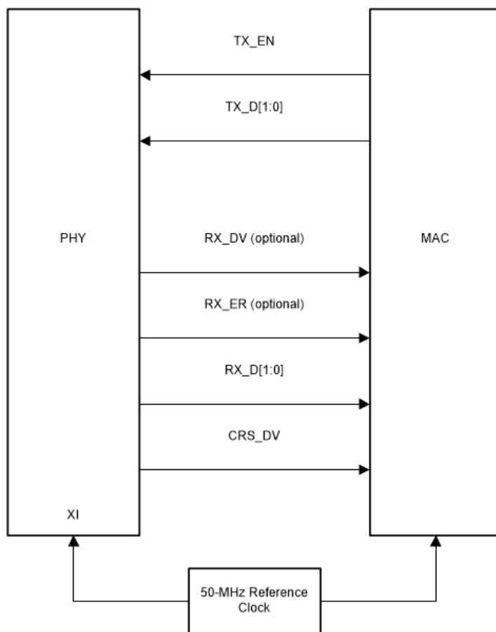
Figure 6-2. RMII Slave Signaling
