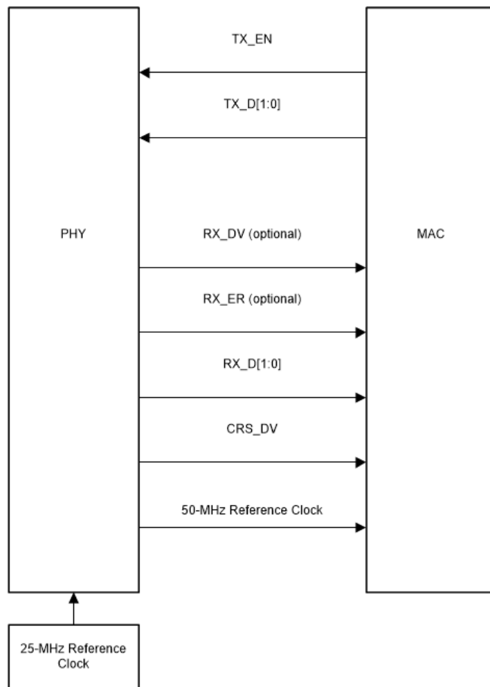
Figure 6-3. RMII Master Signaling
