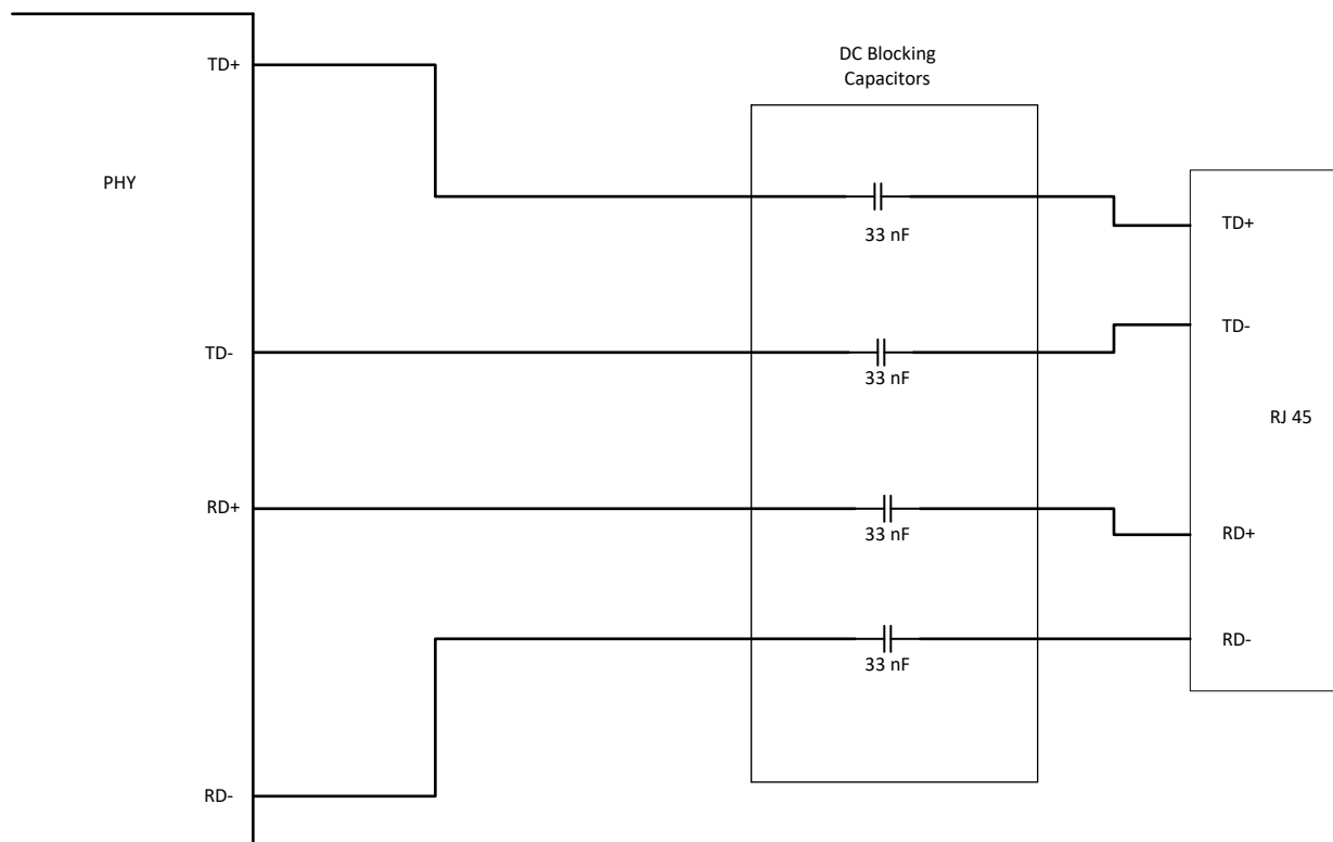
Figure 7-7. Transformer-less DC Blocking Configuration
