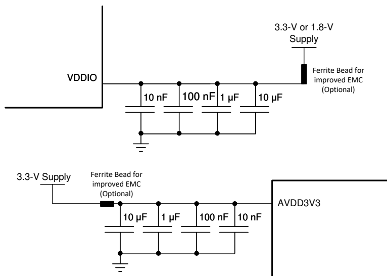
Figure 7-4. DP83825I Power Supply Decoupling Recommendation
