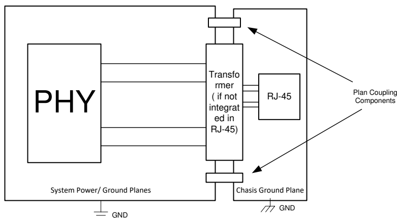
Figure 7-9. Layout Example
