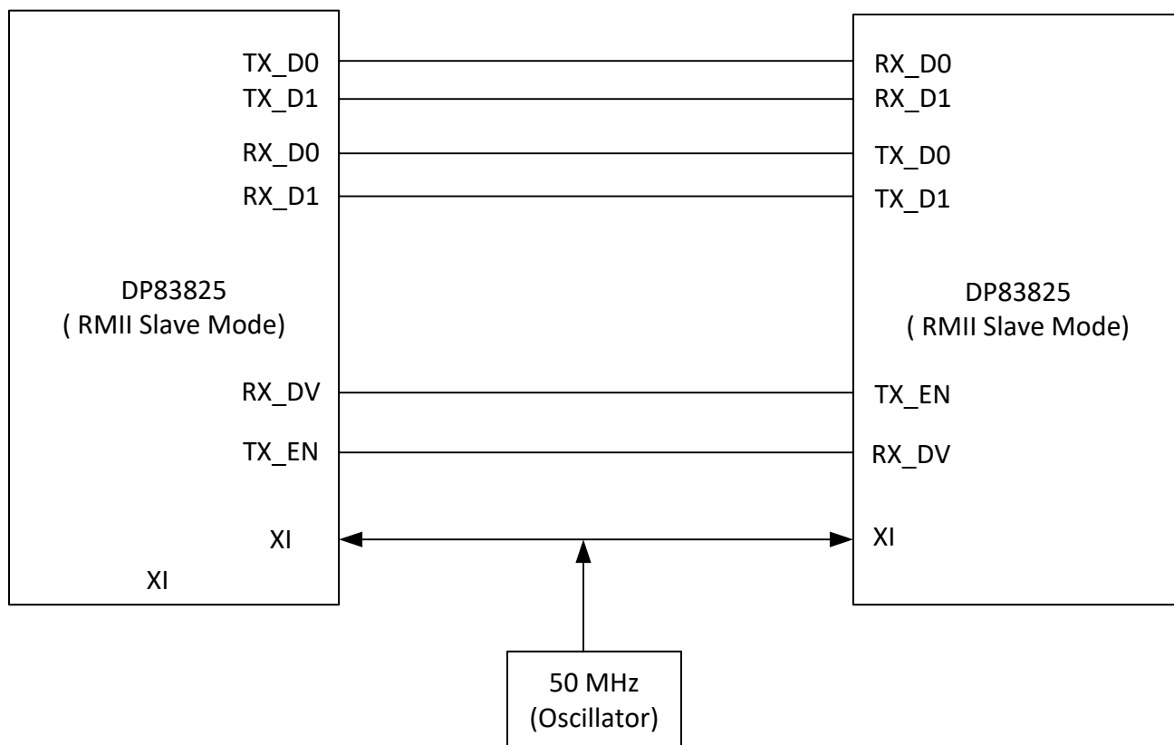
Figure 6-4. RMI Repeater Mode
