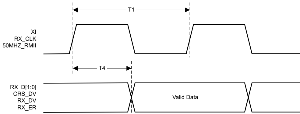
Figure 7-5. RMIITransmit Timing
