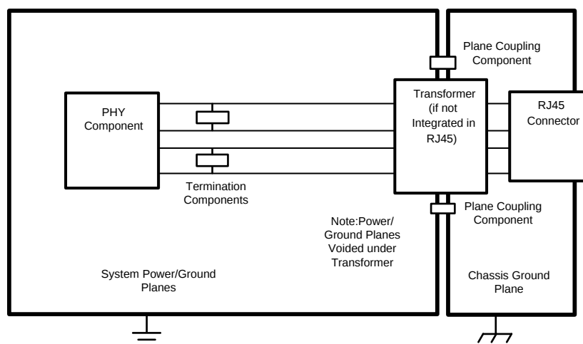
Figure 8-5. Layout Example
