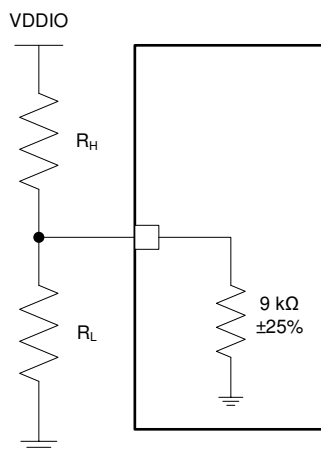
Figure 7-14. Strap Circuit
