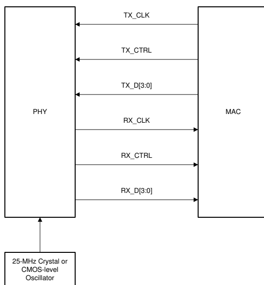
Figure 7-12. RGMII Connections
