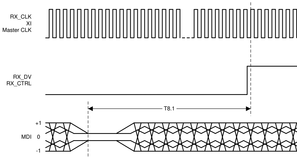
Figure 7-4. Receive Latency
