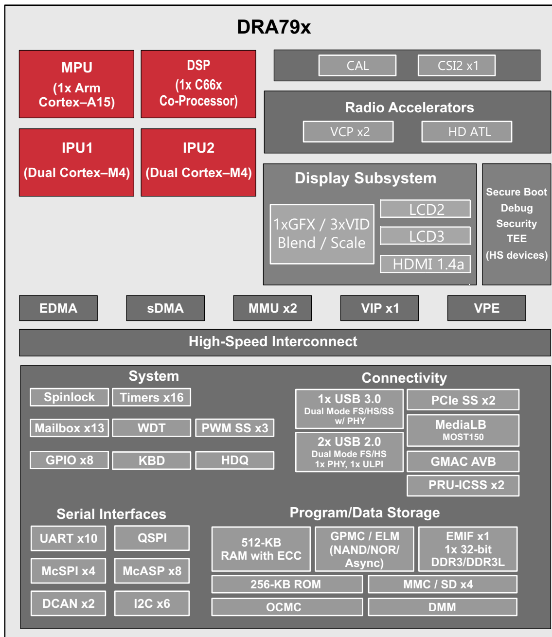
Figure 6-1. DRA79x Block Diagram
