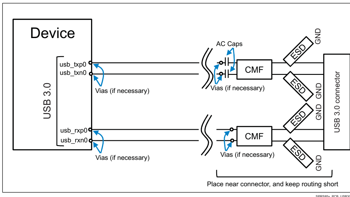
Figure 7-30. USB 3.0 Interface High Level Schematic
