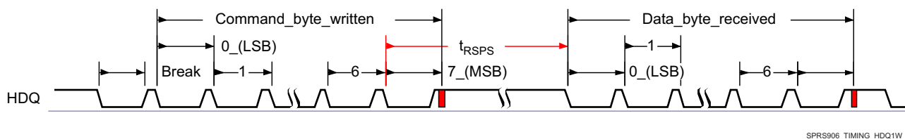
Figure 5-44. HDQ Communication Timing
