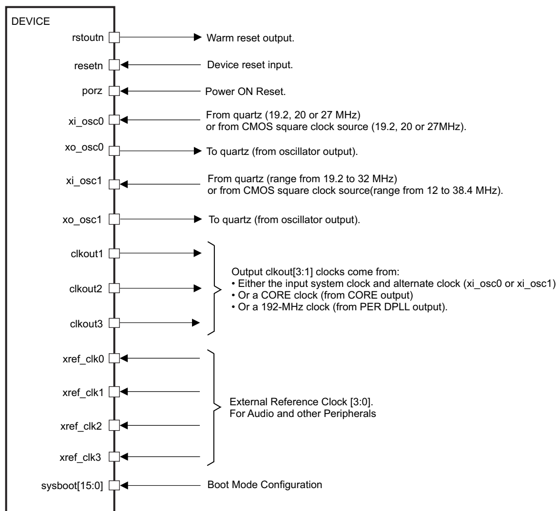
Figure 5-11. Clock Interface
