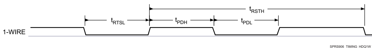
Figure 5-45. 1-Wire—Break (Reset)
