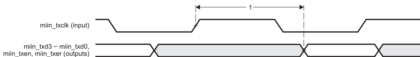
Figure 5-71. GMAC Transmit Interface Timing MIIn operation
