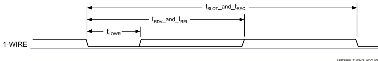
Figure 5-46. 1-Wire—Read Bit (Data)
