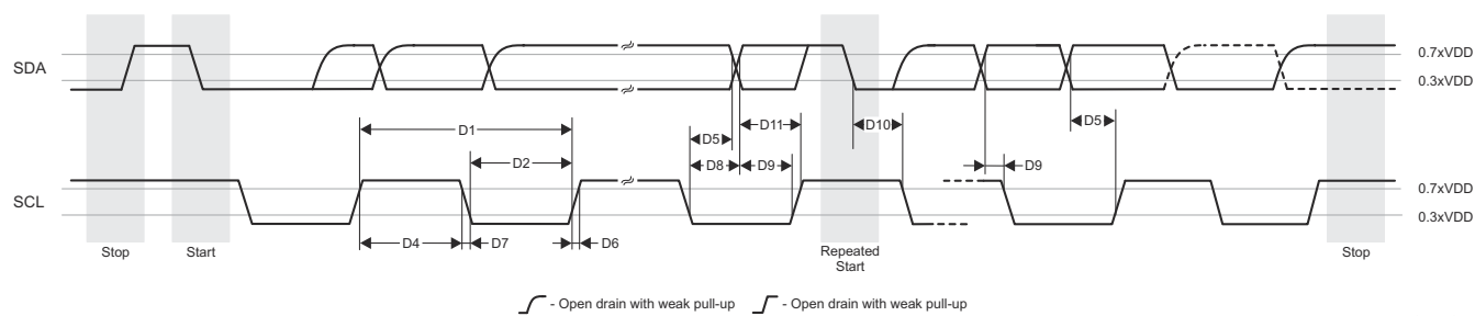
Figure 6-78. I3C Push-Pull Timing (SDR and HDR-DDR Modes)
