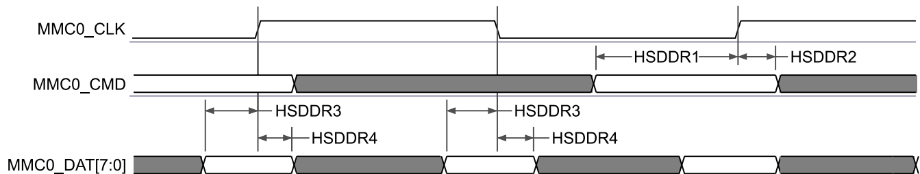
Figure 6-89. MMCSD0 – High Speed DDR Mode – Receive Mode
