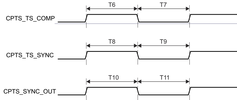
Figure 6-106. CPTS Output Switching Characteristics
