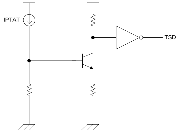
Figure 17. Thermal Shutdown Block Diagram
