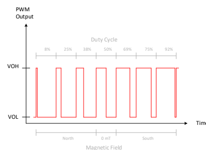
Magnetic Response
