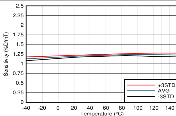
DRV5057Z1, V_{CC} = 3.3 V
