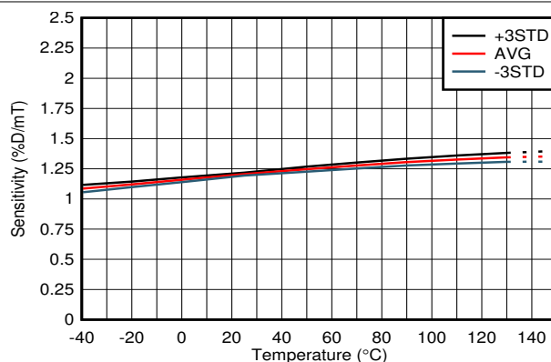
DRV5057A1, V_{CC} = 3.3 V
