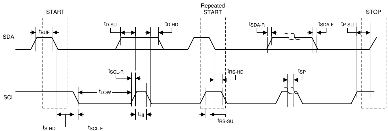
Figure 7-2. I²C Communication Port Timing Diagram
