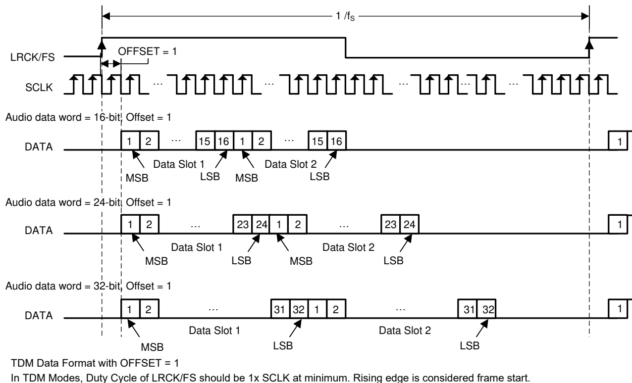
Figure 8-6. TDM 2 Audio Data Format
