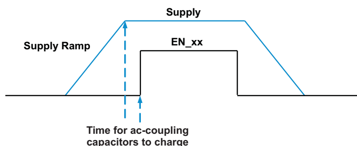
Figure 16. Power-Up/Down Sequence
