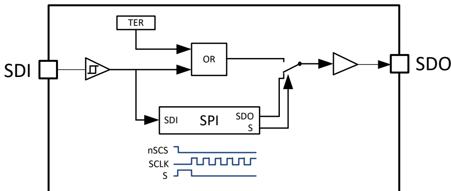
Figure 7-23. Combinational Logic for TER bit
