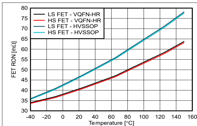
Figure 6-12. R_{HS\_ON} & R_{LS\_ON} vs Temperature at V_{VM} = 13.5 V
