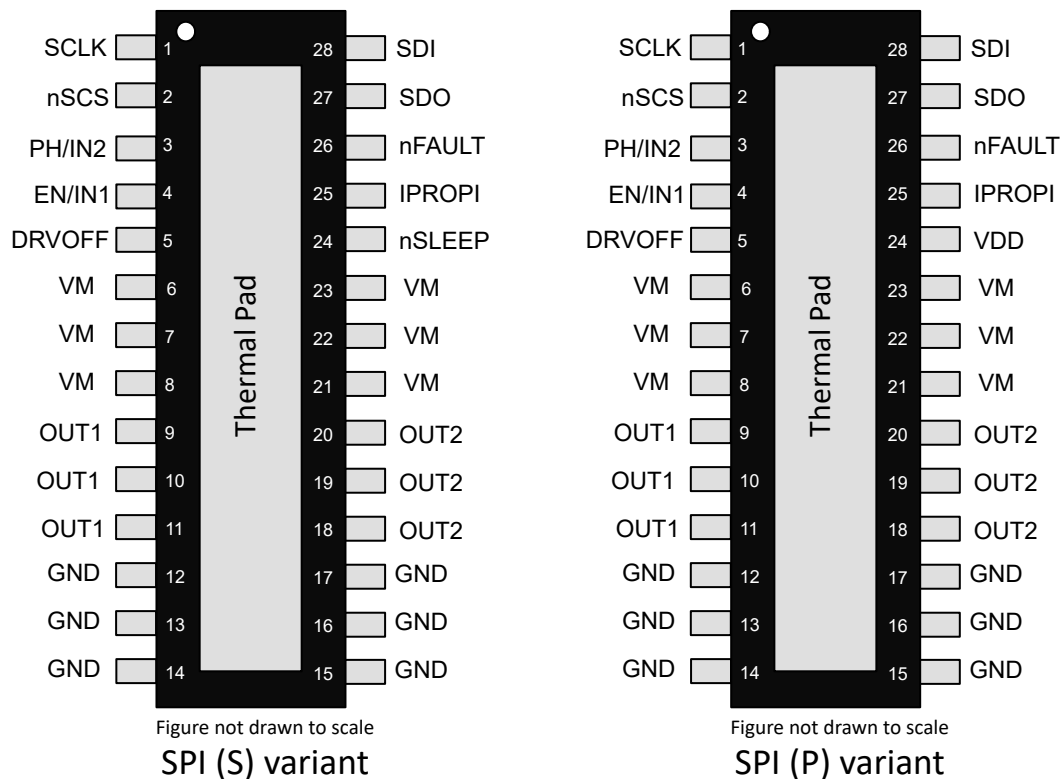
Figure 5-3. DRV8243S -Q1 SPI variant in HVSSOP (28) package
