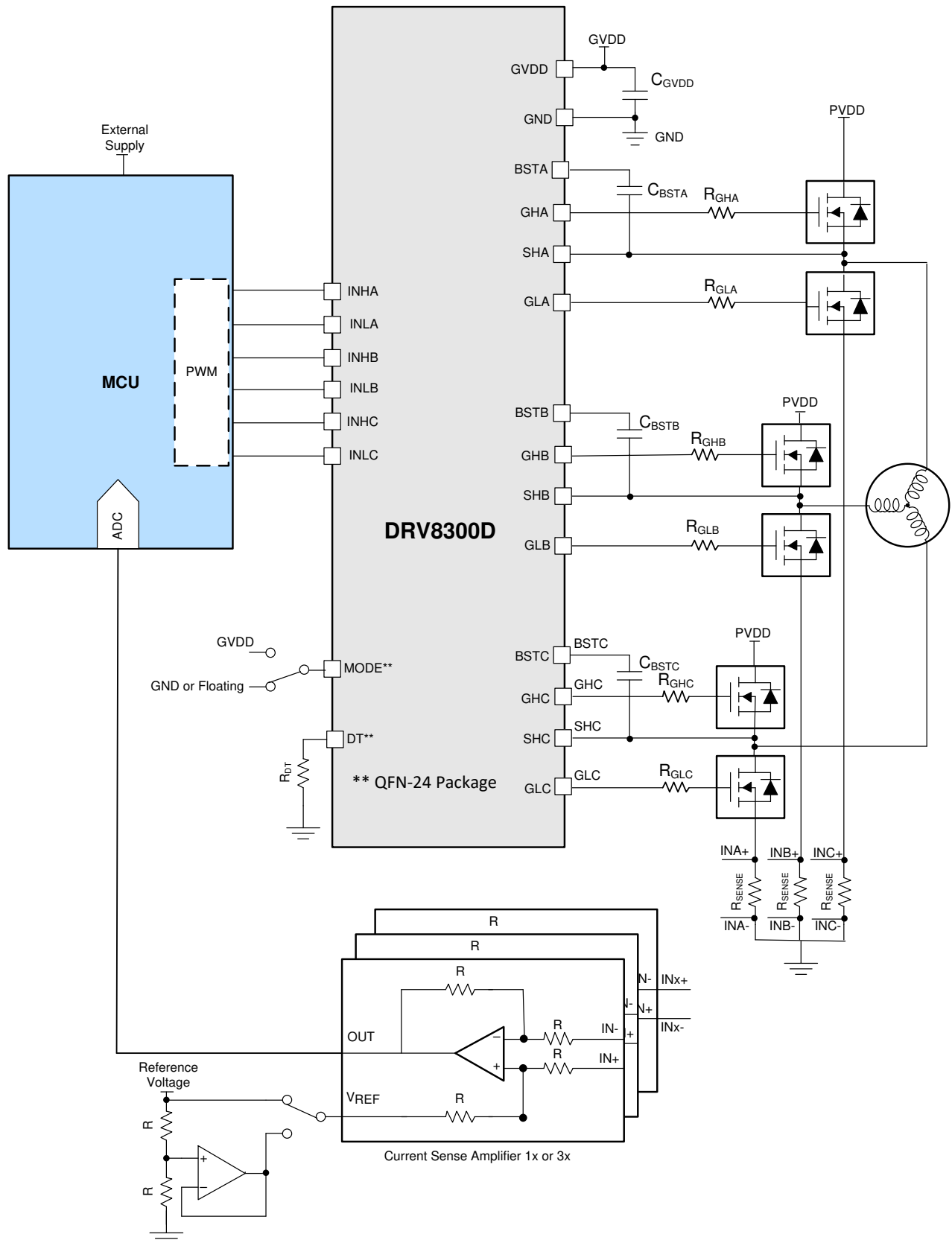
Figure 8-1. Application Schematic
