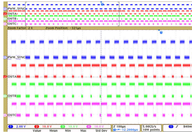
Figure 10-7. PWM Synchronous Duty Cycle Operation with PWM_SYNC = 2b (10% - 90%) (PWM_SYNC, OUTA, OUTB, OUTC)
