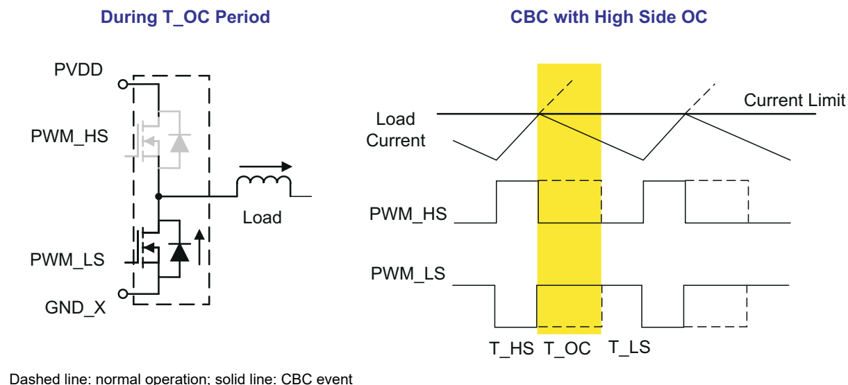
Figure 7-1. Cycle-by-Cycle Operation With High-Side OC
