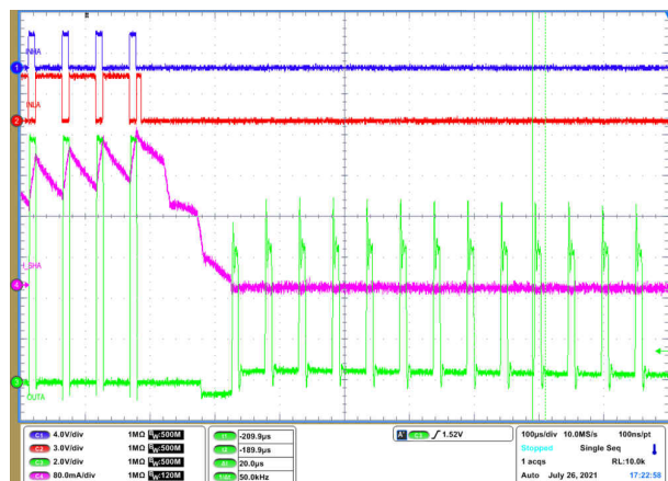
Figure 9-8. Driver PWM with active demagnetization (ASR and AAR)
