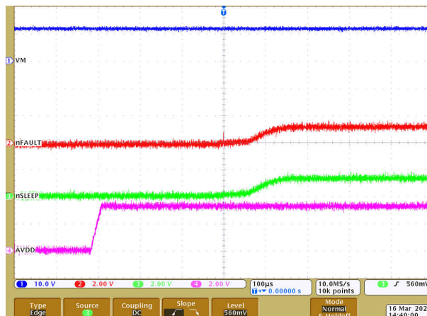
Figure 9-5. Device powerup with nSLEEP
