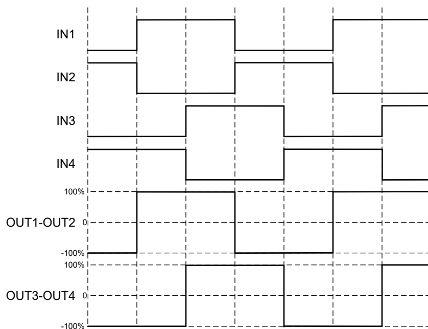
Figure 7-4. Full-Step Mode
