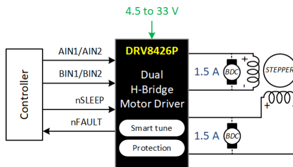
DRV8426P Simplified Schematic
