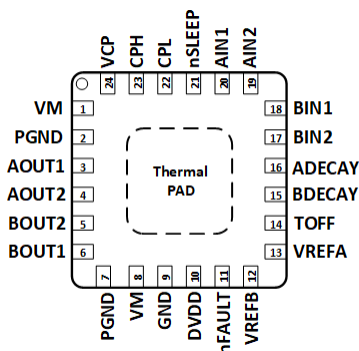
Figure 5-4. RGE Package 24-Pin VQFN with Exposed Thermal PAD Top View DRV8426P
