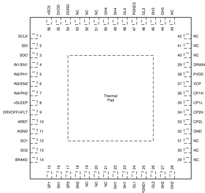
Figure 5-8. DRV8714S-Q1 VQFN (RVJ) 56-Pin Package Top View
