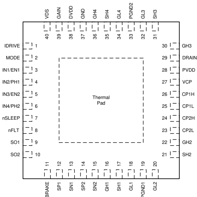
Figure 5-10. DRV8714H-Q1 VQFN (RHA) 40-Pin Package Top View
