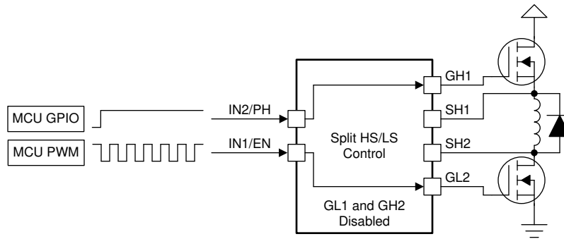
Figure 7-10. Solenoid Control Example
