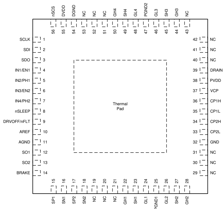
Figure 5-2. DRV8714S-Q1 VQFN (RVJ) 56-Pin Package Top View
