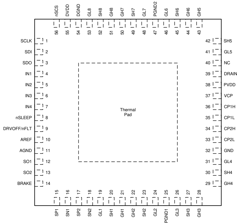
Figure 5-7. DRV8718S-Q1 VQFN (RVJ) 56-Pin Package Top View
