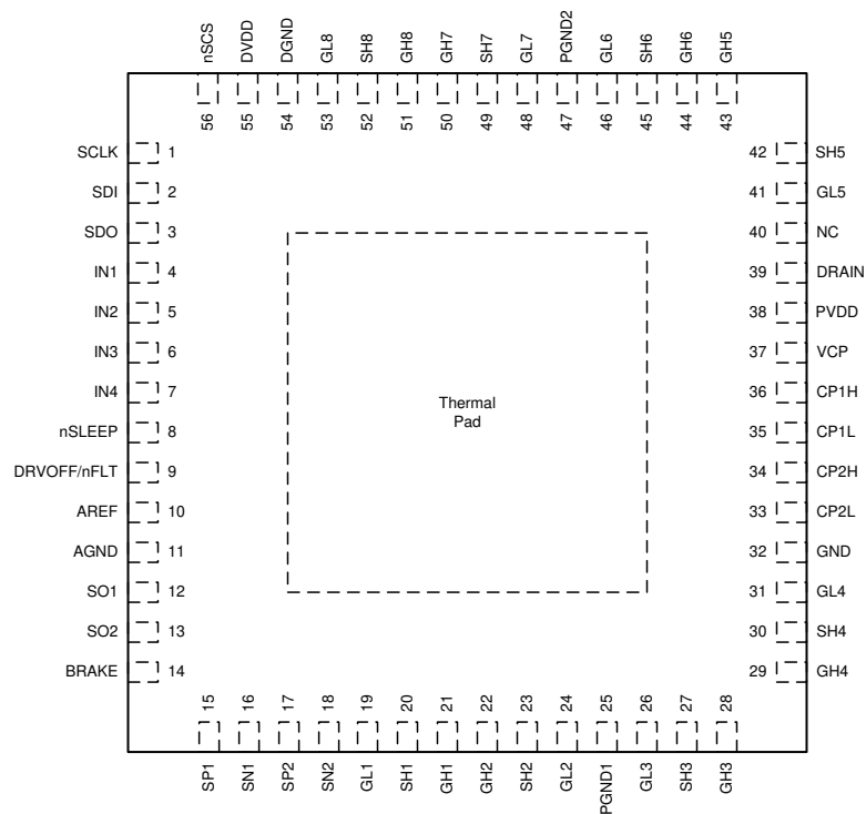
Figure 5-1. DRV8718S-Q1 VQFN (RVJ) 56-Pin Package Top View
