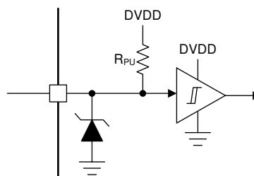
Figure 7-23. Input Pin Structure (nSCS)
