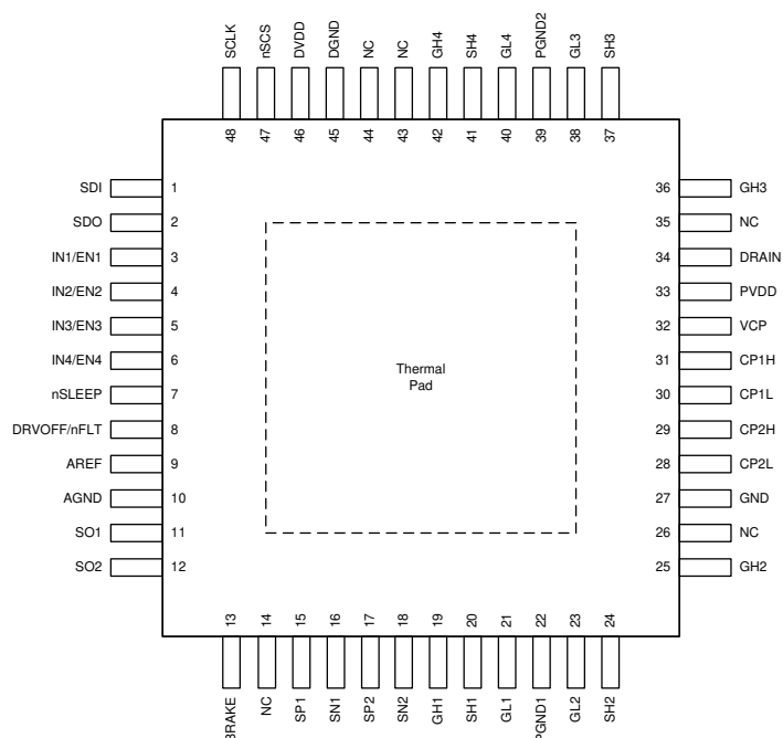
Figure 5-11. DRV8714S-Q1 HTQFP (PHP) 48-Pin Package Top View
