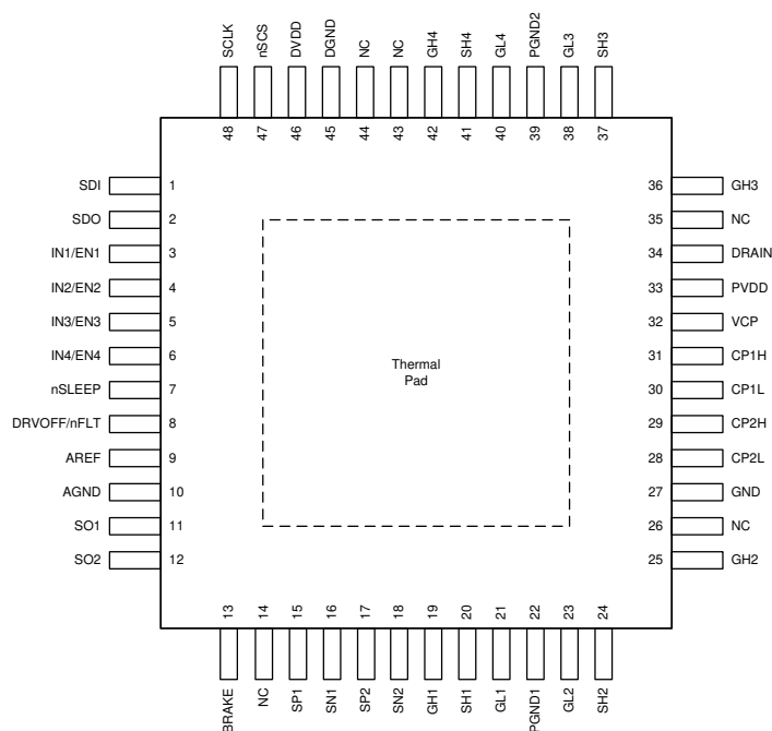
Figure 5-5. DRV8714S-Q1 HTQFP (PHP) 48-Pin Package Top View
