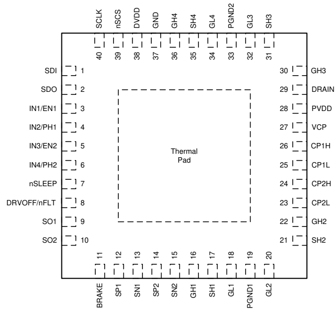
Figure 5-9. DRV8714S-Q1 VQFN (RHA) 40-Pin Package Top View
