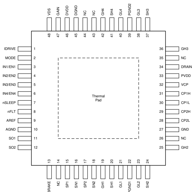
Figure 5-12. DRV8714H-Q1 HTQFP (PHP) 48-Pin Package Top View
